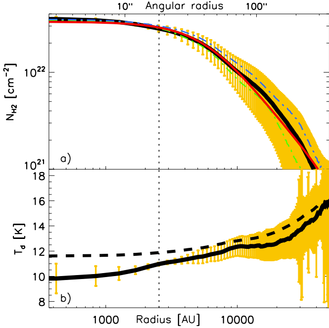
Fig. 4. a) Column density profile of L1689B obtained at 500 \mu\text{m} resolution by applying the Abel reconstruction method to the circularly averaged intensity profiles between 160 \mu\text{m} and 500 \mu\text{m} (solid black curve). The dash-dotted blue and green profiles show the column density profiles obtained from reconstructing the intensity profiles observed along EW and NS sectors, respectively. The overplotted solid red line shows the best-fit Bonnor-Ebert model (see Table 2 for parameters). The vertical dotted line is same as in Fig. 2. b) Reconstructed dust temperature profile of L1689B (solid curve) compared with the LOS-averaged temperature profile derived from simple SED fitting (thick dashed curve).
