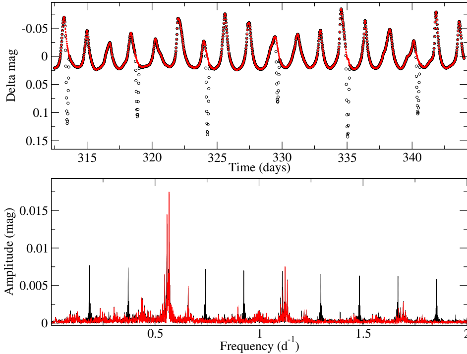
Fig. 4. Upper panel: resulting light curve after iterative removal of the orbital variability (in red) with the original light curve shown for comparison (in black). Lower panel: amplitude spectrum of the original Kepler light curve (in black) and the amplitude spectrum of the pulsation “residuals” (in red) after iterative removal of the orbital variability.
