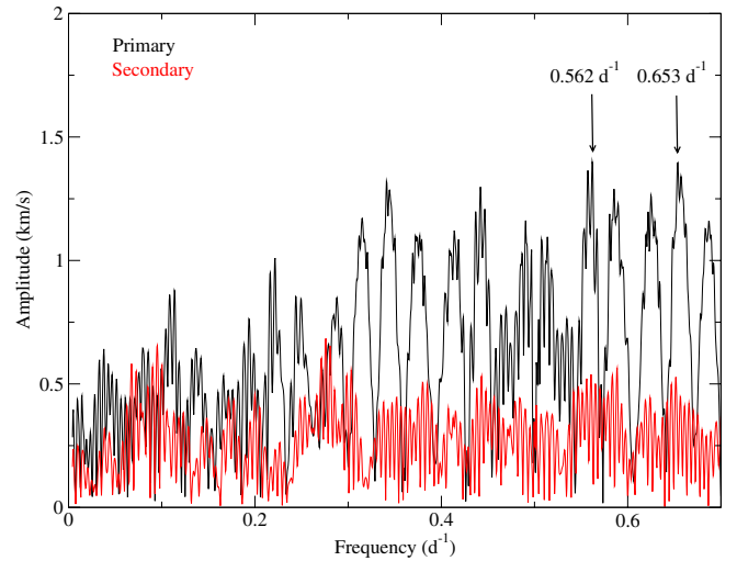
Fig. 9. Amplitude spectrum of the RV residuals for both components after subtraction of the best Keplerian orbit fit. The two highest peaks for the primary (indicated) correspond to frequencies detected in the Kepler light curve.
