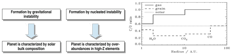
Fig. 9 Left : expected differences in the atmospheric composition due to different formation scenarios. Right : Locations of the ice-lines and their influence on the C/O ratios for the gas and solids (adapted from [120])
