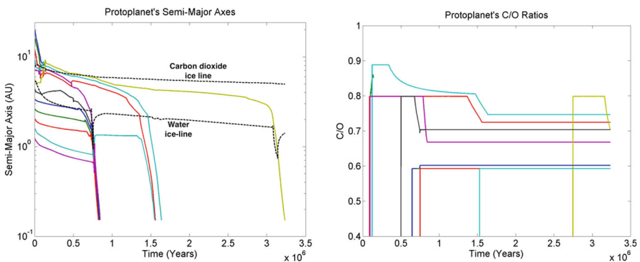
Fig. 10 Left panel : migration trajectories of forming planets. Right panel : Corresponding C/O ratios of planetary envelopes as they accrete and migrate. Note the initially high C/O ratios of planets forming beyond \text{CO}_2 ice-line and reductions in C/O as planets migrate inward where the local disc gas C/O ratio is close to the solar value of \sim 0.54 . Images taken from Coleman & Nelson [44]
