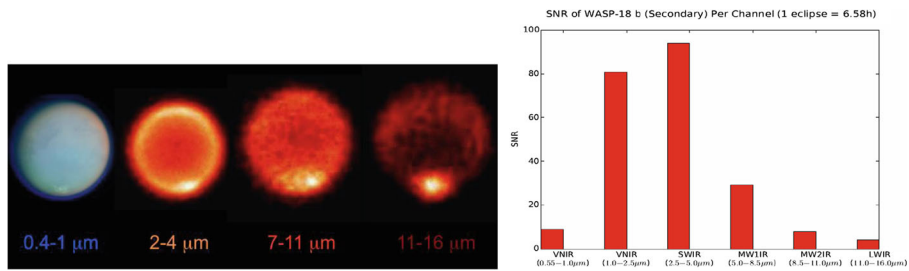
Fig. 8 Left : Demonstration of possible results from exo-cartography of a planet at multiple photometric bands. Right : simulations of EChO performances for the planet WASP-18b: the SNR in one eclipse is high enough at certain wavelength to allow one to resolve spatially the planet through eclipse mapping
