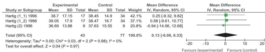
Figure 7. Forest plot showing meta-analysis for SMT: percentage error (accuracy).
