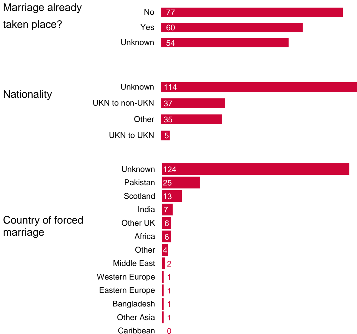
Figure 4 – Case characteristics
