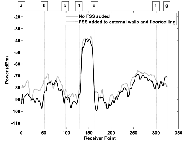
Fig. 17. Comparison of different cases at 5.2 GHz
