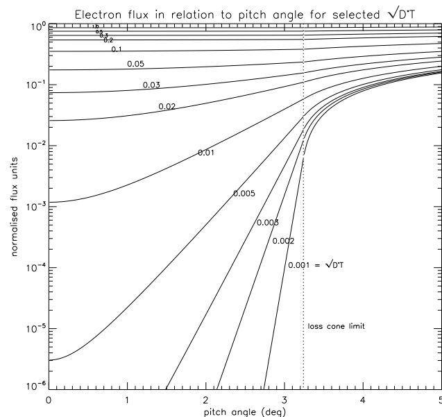
Fig. 7. Electron flux in relation to pitch angle for selected values of diffusion parameter (after Kennel and Petschek, 1966).
