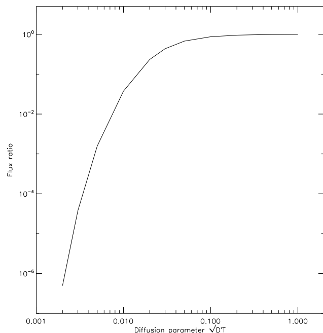
Fig. 8. Ratio between precipitated and trapped electron fluxes (each integrated across their respective detectors) as a function of diffusion parameter.
