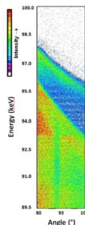
Figure 1. Two-dimensional MEIS spectra obtained from the clean five-fold i -Ag-In-Yb surface.
