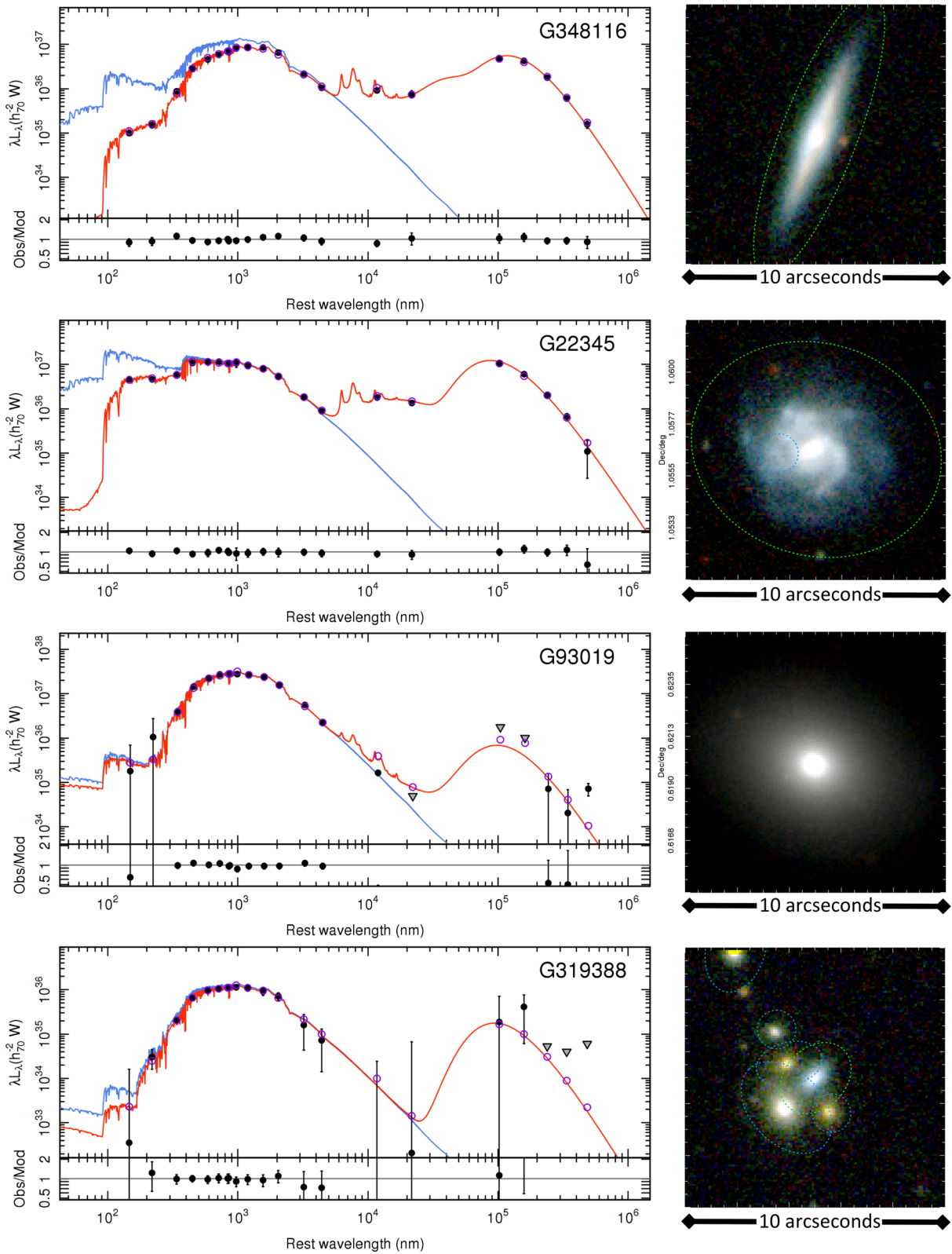
Figure 5. Four examples of GAMA galaxies at z \approx 0.1 processed with MAGPHYS. The left-hand panels show the SEDs showing the data points (black circles), limits (triangles), and the dust attenuated (red curve) and dust unattenuated (blue) MAGPHYS fits, with residual values shown at the bottom. The right-side panels show a KZr images from VISTA/VIKING and SDSS, the green dotted ellipses denote the apertures used by LAMBDA.
