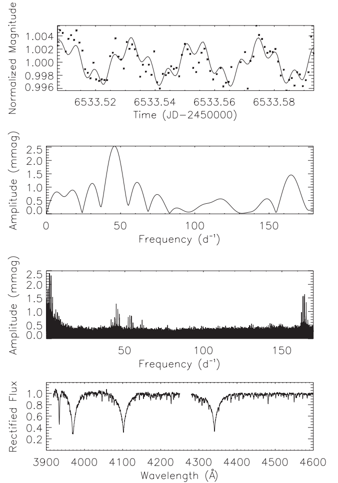
Figure 22. Top: two hours of TRAPPIST follow-up observations confirm the pulsations originate on J1917 (the data have been binned on \sim 1 \text{ min} intervals). Second: periodogram of the TRAPPIST data. The peak at 45 \text{ d}^{-1} is stronger than in the WASP periodogram as there are many pulsations contributing power that are not resolved in just 2 h. The high frequency is at about the same amplitude as the WASP data. Third: the WASP periodogram of J1917 for comparison. Bottom: SALT/RSS spectrum of J1917 showing it to be an A7m star.
