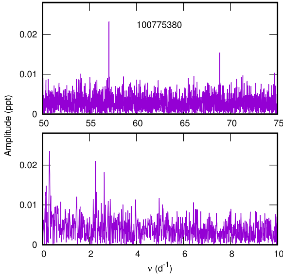
Figure 20. Periodograms of TIC 100775380 in two different frequency regions.
