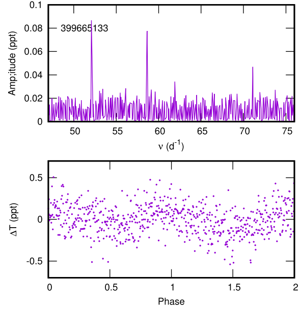
Figure 22. Periodogram of TIC 399665133 in the high-frequency region. No other peaks are visible except for a single low-frequency peak at \nu_{\text{rot}} = 2.237 d ^{-1} . The light curve phased with \nu_{\text{rot}} is shown in the bottom panel.
