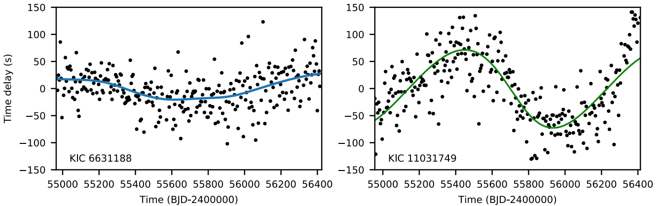
Figure 14. Left-hand panel: Observed time delay for KIC 6631188. The time delay, \tau , is defined such that it is negative when the pulsating star is nearer to us than the barycentre of the system. The blue line is not an orbital solution fit, but rather the time delay as obtained by binning the signal for clarity. If the observed signal is truly periodic, it appears to be on a time-scale longer than the LC data. Right-hand panel: Observed time delays (black dots) and the fitted model (green line) for KIC 11031749. The phase modulation suggests a binary system of low eccentricity, whose orbital period is comparable to or longer than the time-base of the LC photometry.
