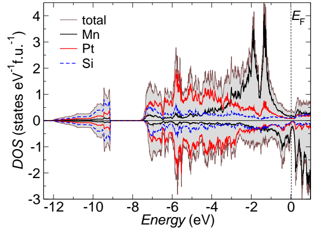
FIG. 10. (Color online) The total and atomic resolved DOS for MnPtSi calculated assuming the FM state. The majority (minority) spin was plotted upward (downward).
