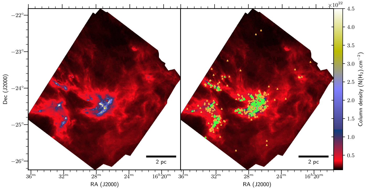
Fig. 2. (Left) Herschel column-density map of the Ophiuchus molecular cloud at an effective HPBW resolution of 18.2''. The column-density map is given in units of \text{H}_2.\text{cm}^{-2} , calculated on a pixel-by-pixel basis using a multi-scale graybody fitting procedure (see Appendix A of Palmeirim et al. 2013 ). (Right) Same as the left panel with the candidate prestellar cores identified in Sect. 4.4 overlaid as green triangles and the unbound starless cores as orange triangles. The bar at the lower right indicates a scale of 2 pc.
