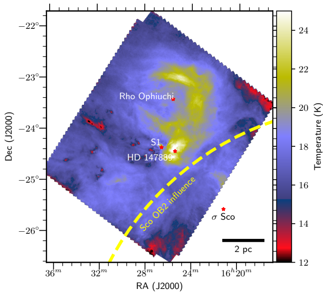
Fig. 3. Herschel dust temperature map of the Ophiuchus molecular cloud at a HPBW resolution of 36.3''. The dust temperature was derived by SED fitting from 160 \mu\text{m} to 500 \mu\text{m} . The warmest regions are located around S1, east of Oph A, and HD 147889, while the warm shell to the northwest is driven by the star \rho Ophiuchi. These three objects are B-type stars, S1 and HD 147889 being both young members of the L1688 infrared star cluster.
