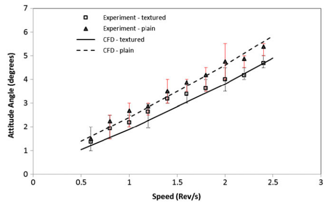
FIGURE 7 Changes in attitude angle over a range of speeds for a load of 1.4 kg (CFD and experimental results). CFD indicates computational fluid dynamics [Colour figure can be viewed at wileyonlinelibrary.com ]
