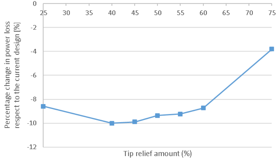
Figure 9: Percentage change in power loss with respect to the current design for 25% - 75% tip relief amount (with surface roughness of 1.6 \mu m)
