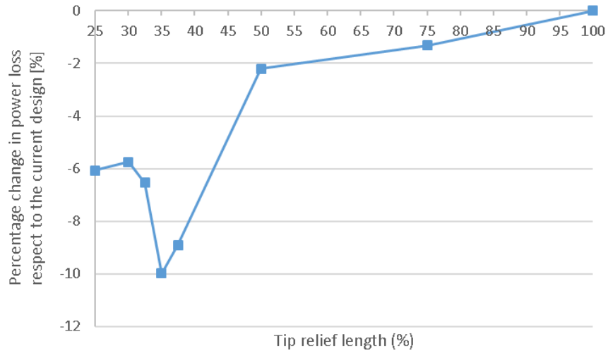
Figure 13: Percentage change in power loss with respect to the current design for the 25% - 100% (current design) tip relief length cases surface roughness of 1.6μm
