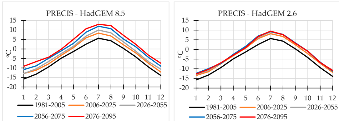
Figure 6. Air temperature scenarios for the study region. Note an increase in air temperature in the first quarter of the century under HadGEM 2.6 scenario and a continuing increase in temperature under HadGEM 8.5 scenario.
