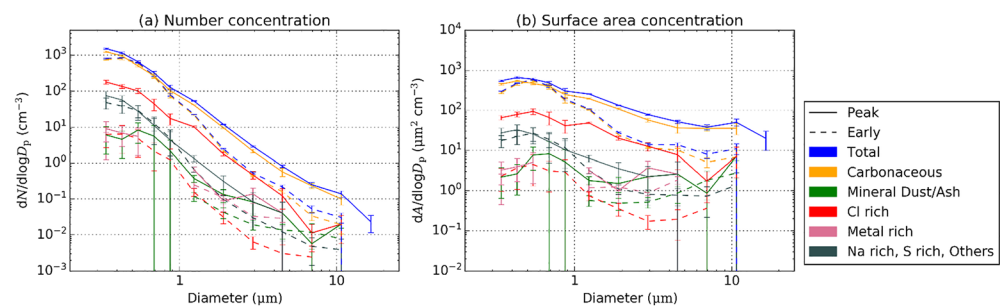
Figure 4. Composition of particles collected on the early (5 November 2017, 16:05–17:25) and peak (5 November 2017, 00:00–00:45) filters in terms of (a) number concentration and (b) surface area. The errors were calculated using Poisson counting statistics. These plots were generated using SEM-EDS analysis.
