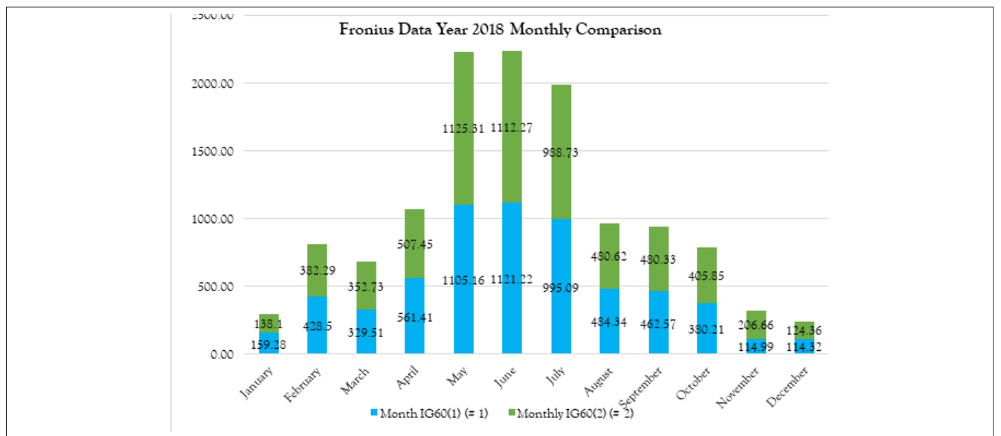
Figure 2: Comparison between outputs of each inverter for each month.
