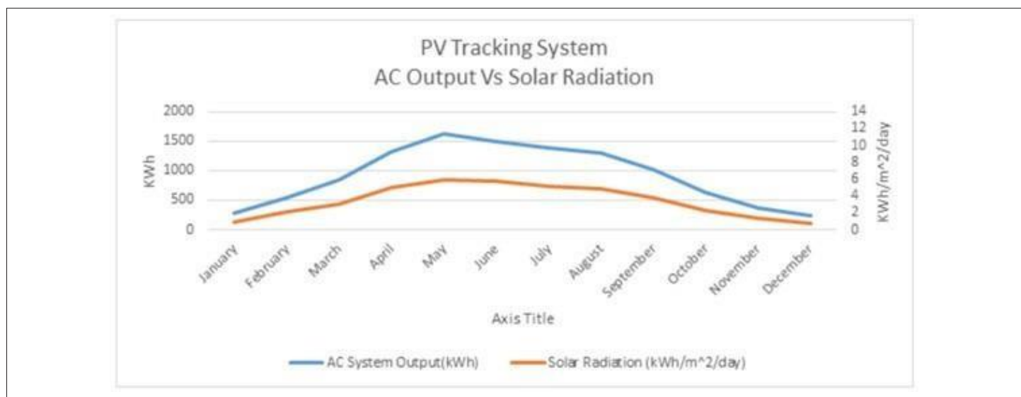
Figure 6: PVWatts Tracking system AC output (blue line) vs Solar Radiation (red line).
