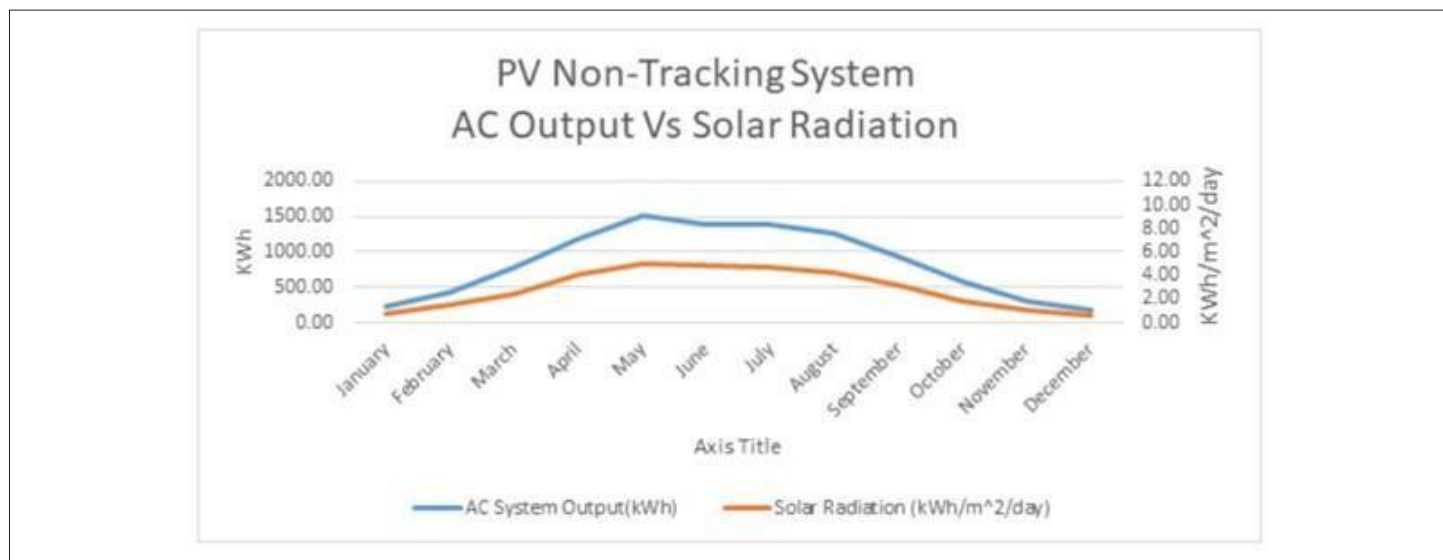
Figure 5: PVWatts Non-tracking system AC output (blue line) vs Solar Radiation (red line).
