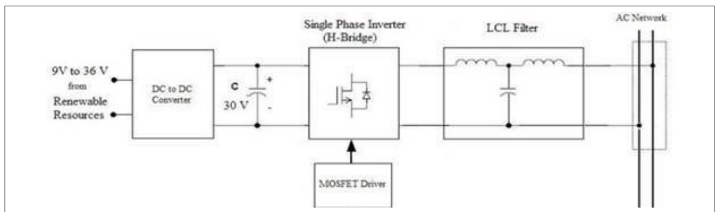
Figure 3: Basic diagram to connect solar panel system to the main grid.
