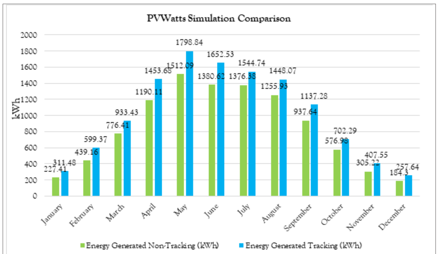
Figure 8: PVWatts simulation model comparison between tracking and non-tracking output.
