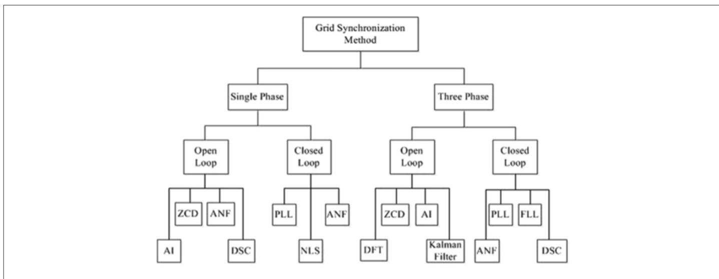
Figure 4: Various grid synchronization methods under respective categories.
