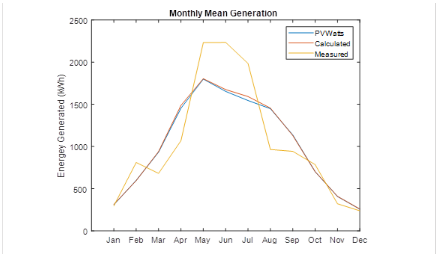
Figure 7: Comparison of mean output for each month between Fronius data (orange line), MATLAB simulation model (red line) and PVWatts simulation model (blue line).
