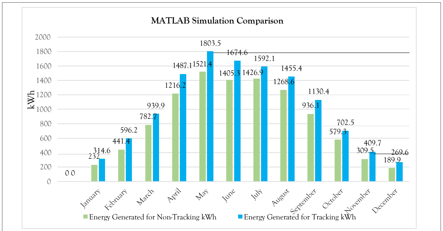
Figure 9: MATLAB simulation model comparison between tracking and non-tracking output.
