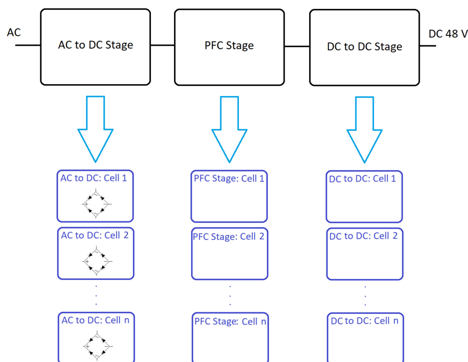
Figure 3. Block diagram of a multicell structure.
