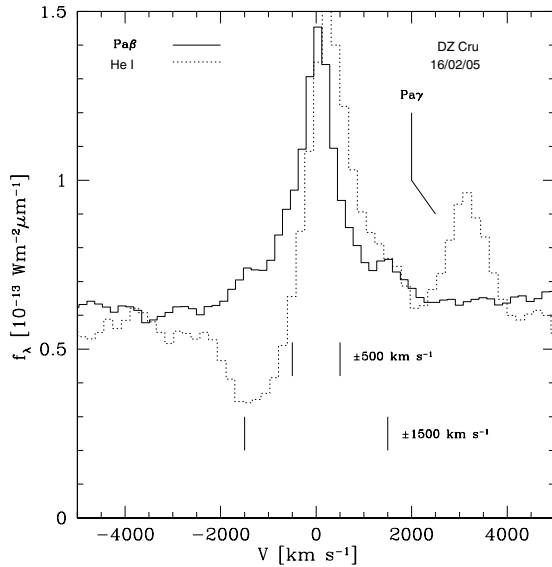
Figure 4. Close up of the Pa \beta line in DZ Cru on 2005 February 16 (solid), showing the line structure, which is similar on all dates of observation. The helium line at 1.083 \mu\text{m} from the same spectrum is shown for comparison (dotted). The emission feature redward of the He I line is Pa \gamma .
