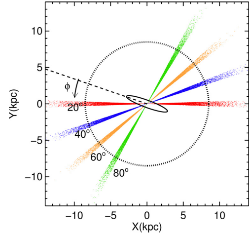
Fig. 4. View of the simulated disc with the different bands selected. The bar is indicated as an ellipse with an orientation of 20 deg with respect to the Sun (at X = -8.5 and Y = 0 ).
