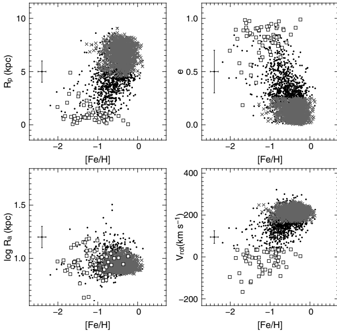
Fig. 6. Perigalacticon, R_p , eccentricity, e , apogalacticon, R_a , and Galactic rotation velocity, V_{\text{rot}} as a function of [\text{Fe}/\text{H}] for the three sub-samples. Symbols are as in Fig. 5. This figure corresponds to Fig. 4 of G03.
