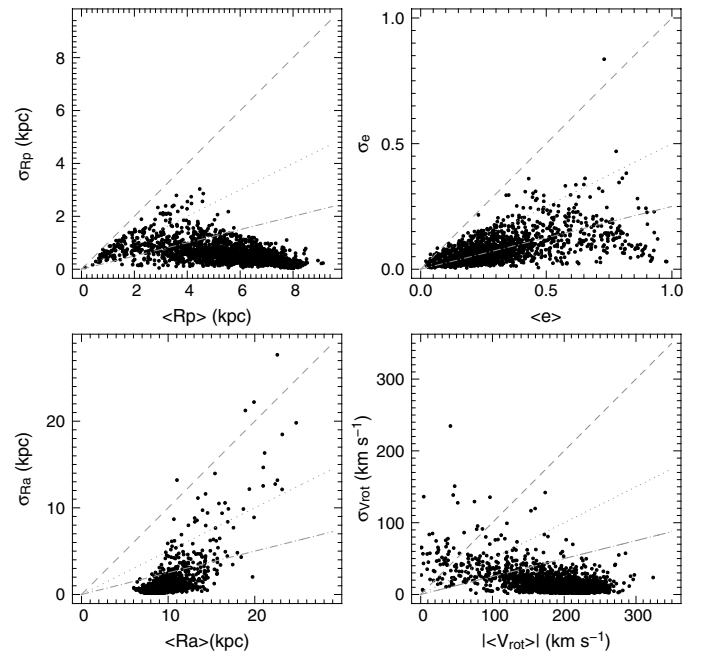
Fig. 3. Estimated uncertainties versus their respective stellar orbital parameters value for the SN75 sample. Dashed, dotted, and dash-dotted lines represent 100%, 50%, and 25% errors, respectively.
