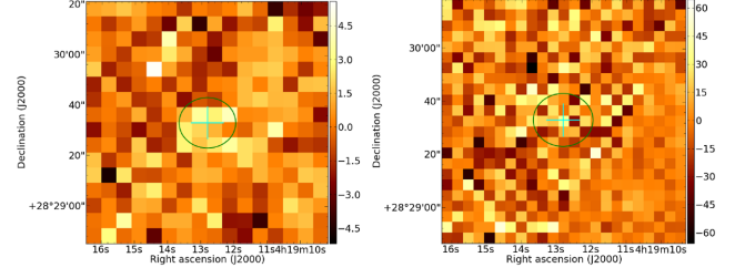
Figure A34. As Fig. A1 FQTauA+B Class II.
