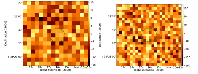
Figure A37. As Fig. A1 J04201611+2821325 Class II.
