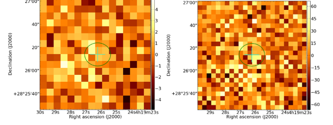
Figure A35. As Fig. A1 V819Tau Class II.
