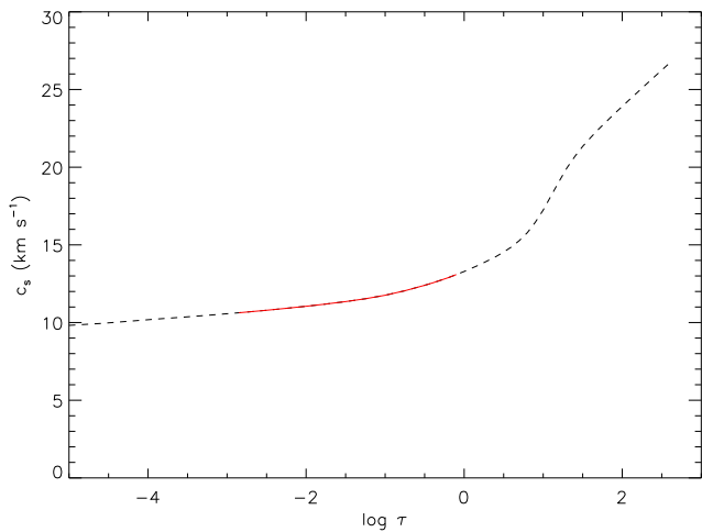
Figure 11. The local sound speed c_s in a hydrostatic LTE model atmosphere for V652 Her at maximum radius as a function of continuum optical depth (broken line). The line-forming region (Fig. 9) is shown as a solid red line.
