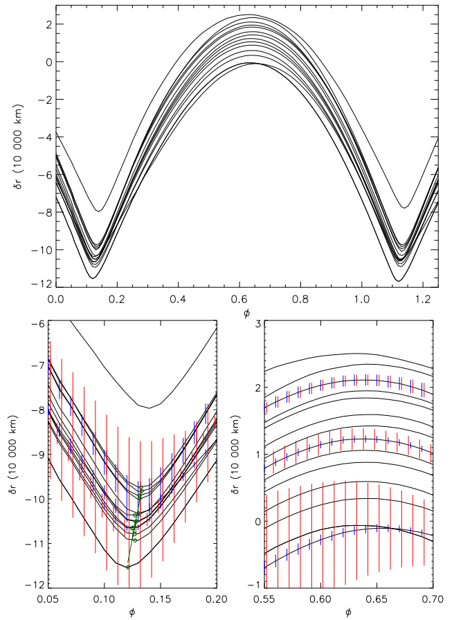
Figure 12. Top: the total radial displacement of different groups of the photosphere of V652 Her as represented by different groups of absorption lines. The lines are grouped by depth of formation at maximum radius into bins with \delta \log \tau_c = 0.2 centred at \log \tau_c = -0.1(0.02) - 2.9 , and normalized using the \tau - z relation shown in Fig. 9 such that a line formed at \tau_c = 0 would have zero displacement at maximum radius. Consequently, the weakest lines correspond to the lowest layers of the photosphere and vice versa. Bottom: expansions of the upper panel around minimum and maximum radius. Since each curve represents the average of several lines within a bin, standard deviations (red) and standard errors in the mean (blue) have been added for three representative bins. The green diamonds represent radius minima for each line group obtained by fitting a parabola through the five points around minimum radius; the solid green line represents a regression on these minima (excluding He I 4471 Å) with a slope d\delta r/d\phi \times d\phi/dt = 141 \pm 17 \text{ km s}^{-1} .
