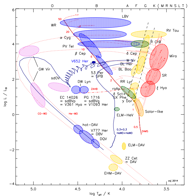
Figure 1. Luminosity–effective temperature (or Hertzsprung–Russell) diagram showing the position of V652 Her (Jeffery, Woolf & Pollacco 2001) and the post-merger evolution track for a double helium white dwarf binary ( 0.3+0.3 M_{\odot} ; thick blue line; Zhang & Jeffery 2012). The latter shows expansion to become a yellow giant following helium-shell ignition. As the helium-burning shell migrates towards the core, the star contracts through a series of loops caused by helium-shell flashes, until it reaches the helium main sequence. On completion of core helium burning, the star returns to the white dwarf cooling track. Although V652 Her is located below the main sequence in the HR diagram, it is spectroscopically a giant; historically, the latter is a spectroscopic term and depends on luminosity-to-mass ratio (or surface gravity). In the case of the 0.6 M_{\odot} V652 Her, this is higher (lower) than for main-sequence stars of the same effective temperature. Also shown are the approximate locations of other pulsating variables coloured roughly by spectral type, the zero-age main sequence and horizontal branch, the Cepheid instability strip, and evolution tracks for model stars of various masses, indicated by small numbers ( M_{\odot} ). Shadings represent opacity-driven p modes (\\), g modes (///) and strange modes (||) and acoustically driven modes (≡). Approximate spectral types are indicated on the top axis. Based on figures by J. Christensen-Dalsgaard and subsequently by Jeffery (2008).
