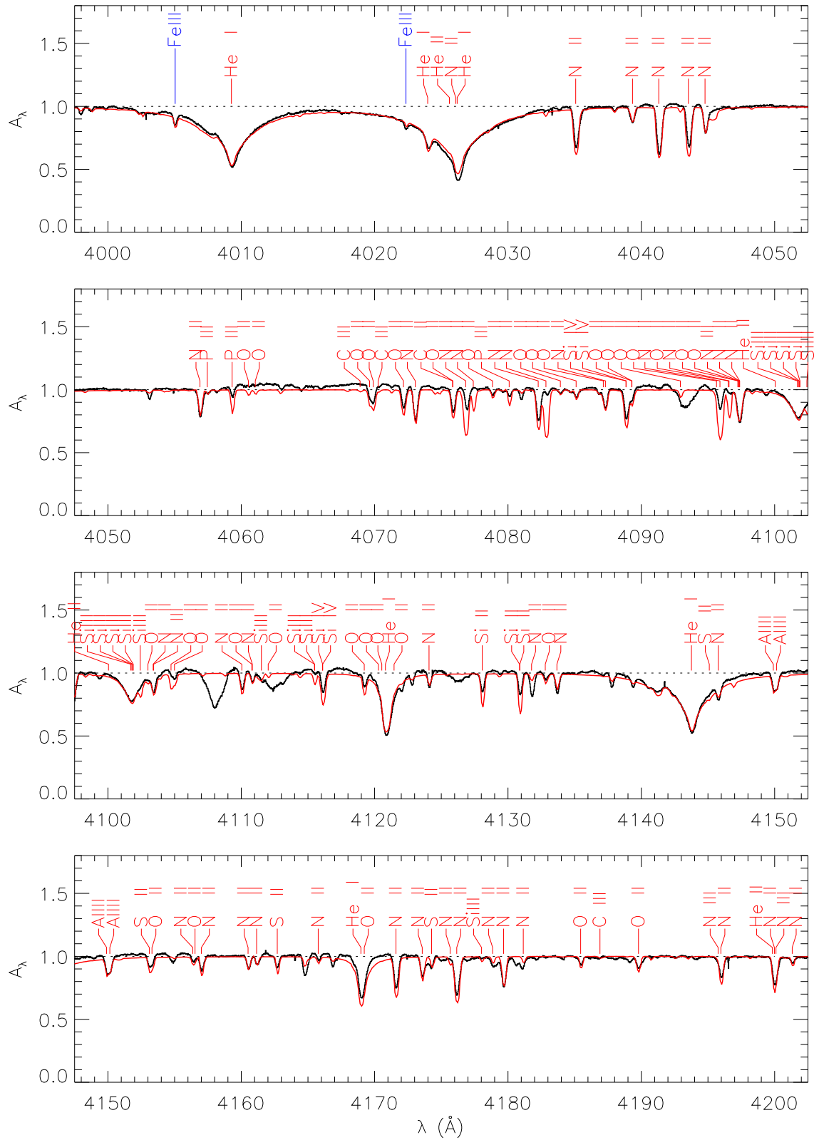
Figure B1. (a) The median Subaru spectrum of V652 Her between phases 0.60 and 0.70 (black), together with an approximate LTE synthetic spectrum computed using the parameters given in Section 5.1 (red). Lines in the model with W_\lambda > 10 mÅ are identified by ion. Ions with Z > 20 are shown in blue. The hydrogen Balmer lines at 4101 and 4340 Å are not labelled but are included in the model. The model continuum is shown as a dotted line. Strong broad features around 4093, 4108, 4112 and 4126 Å are instrumental artefacts.
