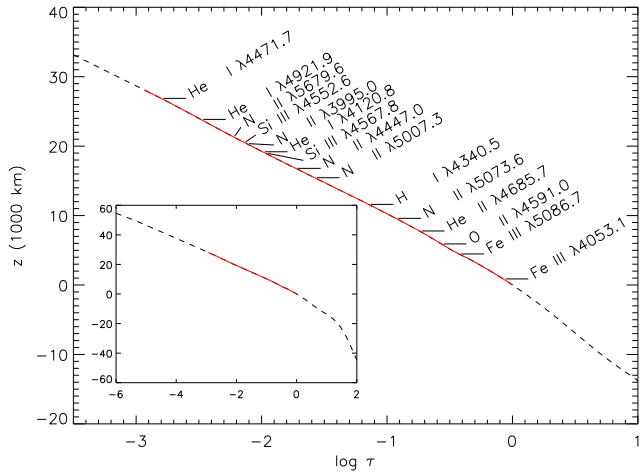
Figure 9. Detail from the run of geometric height above the continuum forming layer z(\tau) - z(1) as a function of optical depth \tau_{4000} in a model for the atmosphere of V652 Her (broken line). The line-forming region is marked as a solid red line. The locations of formation of the cores of the representative lines in Fig. 8 are indicated. The same function for the entire model atmosphere is inset.
