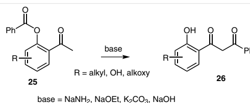
Scheme 5 Typical rearrangement conditions
