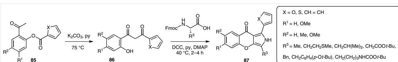
Scheme 19 A heterocyclic Baker-Venkatarman rearrangement
