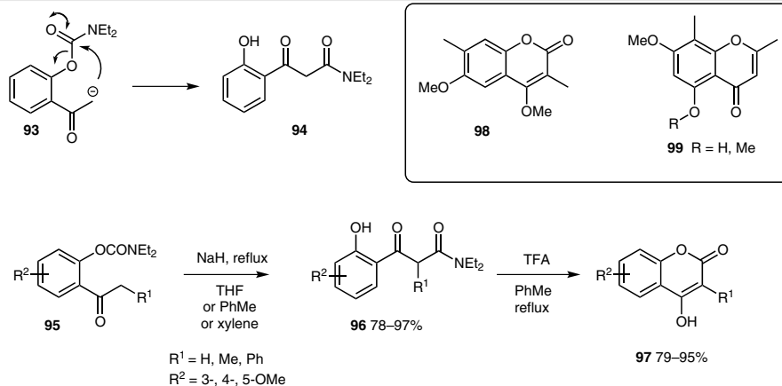
Scheme 21 The synthesis of coumarins and isoeugenetin methyl ether ( 99 )
