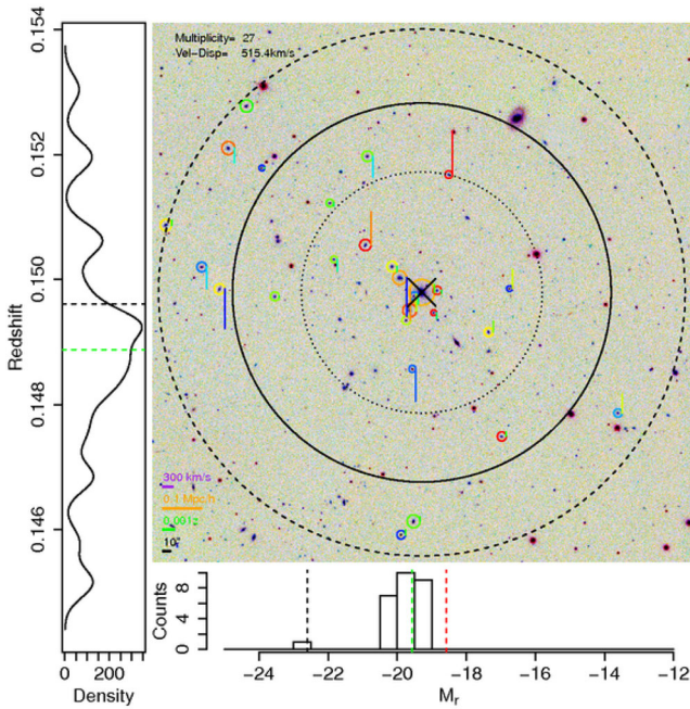
Figure 33. Example group image. The background image is a urK composite. Group members are marked by circles. The size of a circle scales with the galaxy’s r -band flux, while its colour reflects the galaxy’s u - r colour. A galaxy redshifted with respect to the group median redshift has a red upwards pointing line, the length of which scales with the velocity difference, while for a blueshifted one the line is blue and points downwards. The rings represent the 50, 68 and 100 percentiles of the radial galaxy distributions relative to the iterative group centre. The velocity probability density function smoothed with a Gaussian kernel of width 50 \text{ km s}^{-1} (the typical GAMA velocity error) is shown on the left, where the group median is shown with a green dashed line and the BGG with a black dashed line. The bottom panel presents the absolute r -band magnitude distribution of the group, with the effective GAMA survey limit shown with a red dashed line, the group median absolute magnitude with a green line and the BGG absolute magnitude with a black line.
