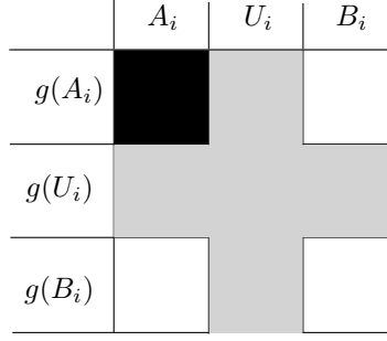
FIGURE 1. The sets A_{i+1} , U_{i+1} and B_{i+1} as intersections of the sets A_i , U_i , B_i , g(A_i) , g(U_i) , and g(B_i) . The set A_{i+1} is represented by black, U_{i+1} by grey, and B_{i+1} by white.
