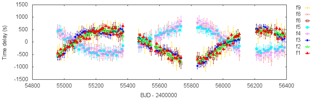
Fig. 3. Time delays for KIC4471379 – a binary with two \delta Sct stars. Time delays show two pseudo-sinusoids with equal periods and opposite phases.
