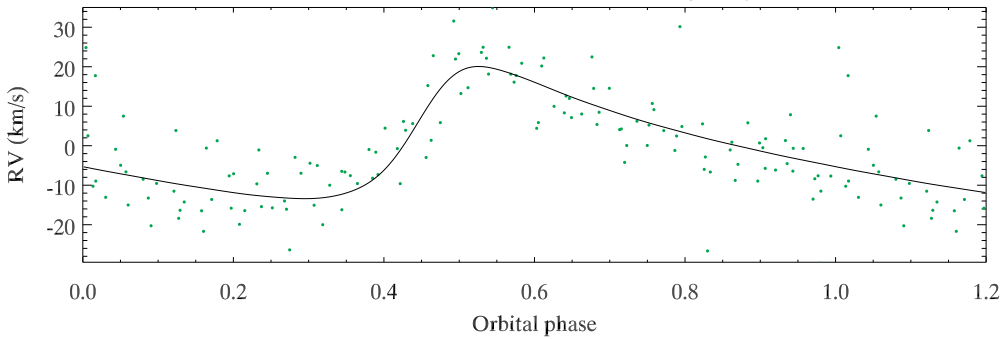
Fig. 2. Phased RV curve for KIC9651065, whose time delays were shown in Fig.2. Green circles represent individual RV measurements, and the black curve is the fit obtained using analytical functions described in [1].
