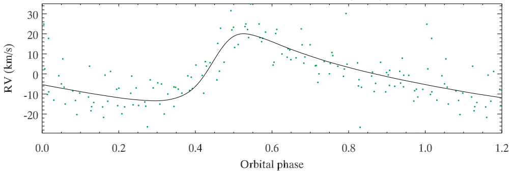
Fig. 2. Phased RV curve for KIC9651065, whose time delays were shown in Fig. 2. Green circles represent individual RV measurements, and the black curve is the fit obtained using analytical functions described in [1].
