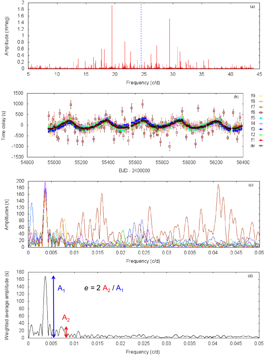
Fig. 1. (a): Fourier transform of the light curve of KIC9651065. The dashed line is the Kepler LC Nyquist frequency. (b) Time delays for the nine highest peaks, using 10-d segments. Nyquist aliases are excluded using the super-Nyquist asteroseismology method ([18]). (c) Fourier transforms of the time delays for those nine peaks; all show variability at the binary orbital frequency \nu_{\text{orb}} = 0.00367 \text{ d}^{-1} . (d) Fourier transform of the weighted-average time-delays. The orbital frequency and two harmonics, which have amplitudes of A_1 = 165.6 , A_2 = 38.4 and A_3 = 10.2\text{s} (\pm 2\text{s}) , were obtained from least squares fitting. The inferred eccentricity is e = 0.46 .
