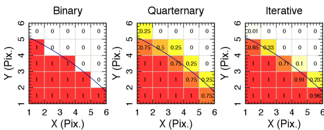
Figure 2. A demonstration of the three types of aperture placement that can be employed in LAMBDA R . The left-hand panel shows how aperture pixels are assigned using the binary aperture placement method; the centre panel shows pixel assignments using the quaternary aperture placement method; and the right-hand panel shows pixel assignments using the recursive descent method, implemented (by default) in LAMBDA R .
