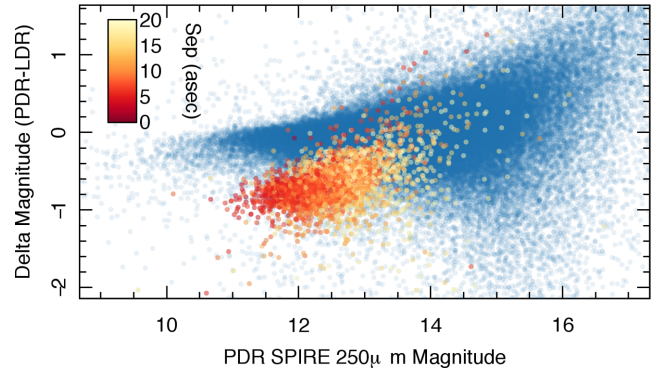
Figure 22. Demonstration that the population of objects offset from 0 in the SPIRE 250 \mu\text{m} trumpet is caused by deblending of nearby contaminants. Here colouring is by separation between the object and its nearest-neighbour contaminant, in arcseconds. The blue points in the background is the distribution of all objects not matched to a contaminant within 20 arcsec, for reference.
