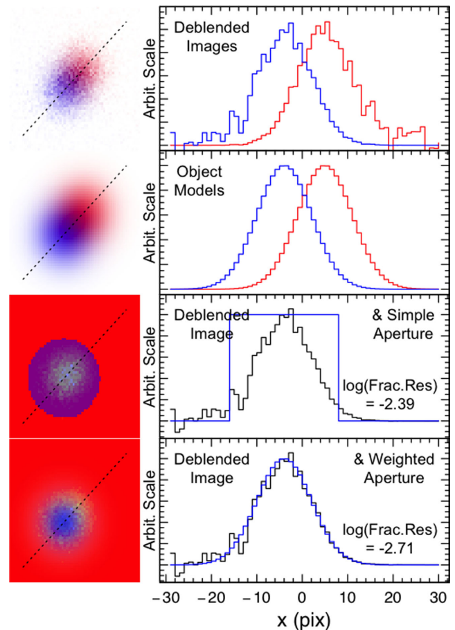
Figure 8. Demonstration of the two different measurement methods, being applied to the simulated objects in Fig. 3. The top panel is the same as the final panel in Fig. 3. The second panel shows models for the two sources. The third panel shows the ‘simple’ measurement aperture for the blue source (after passing the model through the binary filter detailed in Section 3.7), overlaid on the ‘deblended image’ ( I(x, y) \times W(x, y) ) in black. The bottom panel shows the ‘weighted’ measurement aperture, which is identical to the model aperture M(x, y) . Again, this aperture is overlaid on the ‘deblended image’. In the bottom two panels, the text inset shows the fractional residual between the input flux and the flux measured by the aperture after accounting for aperture normalization (Section 3.8). As is discussed in Section 3.4, in practice the program constructs individual ‘deblended apertures’ rather than the ‘deblended images’, shown here, as they are equivalent. We demonstrate deblended images here simply for clarity, to better explain the process.
