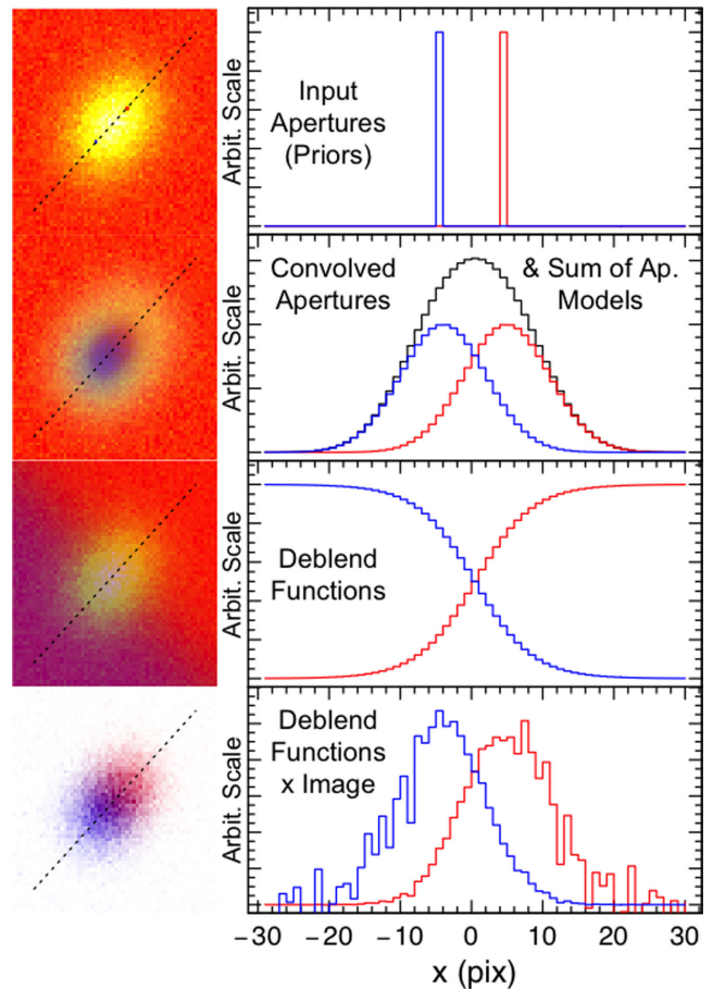
Figure 3. Demonstration of how deblending of apertures is performed. Two point sources (i.e. objects perfectly modelled by the PSF) were simulated using an example PSF and noise profile (image top left). Model parameters for two point sources are provided to the program, at the known locations of the two objects (thereby simulating use of a known optical prior; top right). Using these priors, and the known PSF, models for the two sources are generated (second row). The deblend function for each object is determined by the ratio between each model and the sum of all models (third row). The image is then deblended for each object, through multiplication by the deblend function (fourth row). This final image is then used for flux measurement, using the user-desired measurement method (see Section 3.7). In each row, the right-hand column shows the slice through the left-hand image along the dotted black line.
