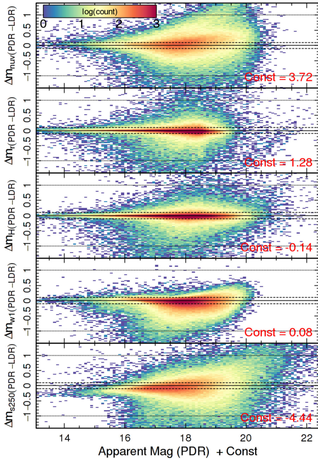
Figure 20. ‘Trumpet’ plots showing difference in magnitude versus PDR magnitude for the GALEX NUV, SDSS r , VIKING H , WISE W1 , and SPIRE 250 \mu\text{m} bands, demonstrating that the photometry is in broad agreement with the PDR photometry, but none the less shows systematic differences caused by subtle differences in measurement methods. Each panel has a horizontal offset applied, which is given in the lower right of each panel. Horizontal dashed and dotted lines are shown at \pm 0.1 and 1 mag, respectively, for reference.
