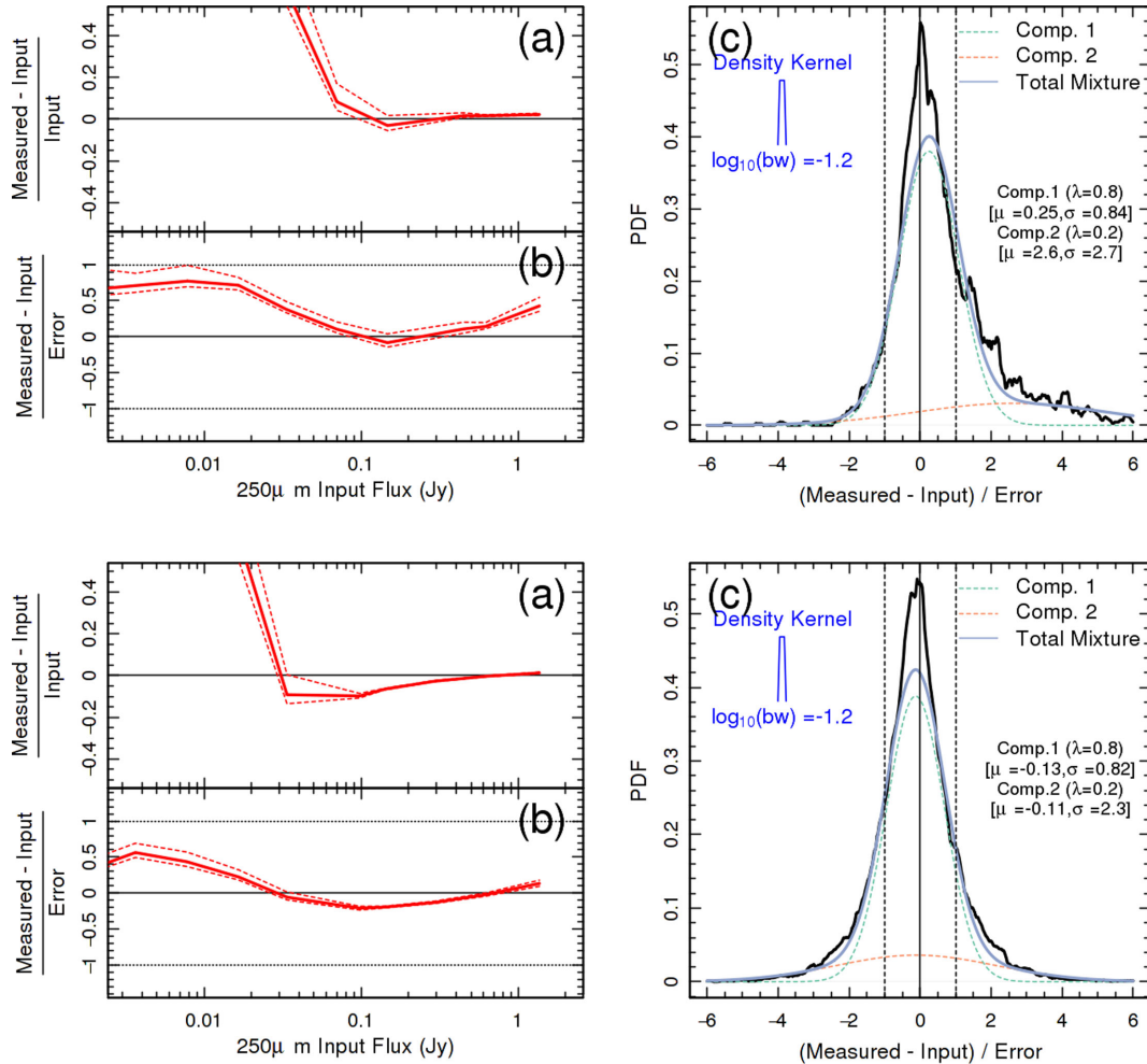
Figure 15. Here we show the same as in Fig. 14, but using contaminant lists cut at 6\sigma (top) and 2\sigma (bottom). From this figure, we can see that the choice of contaminant list depth has important effects: a shallow list creates unwanted flux boosting of faint and bright sources, while a deep list slows convergence and increases shredding of sources, as seen by the systematic suppression of fluxes around 0.1 Jy.
