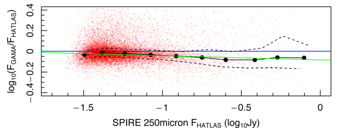
Figure 20. A comparison between the preliminary Herschel -ATLAS 5\sigma catalogue and the optically motivated catalogue derived here in the SPIRE 250 \mu\text{m} band. It should be noted that the zero-points calibration and entire reduction process have evolved between these catalogues. Note units are in Jansky as is standard in the far-IR.
