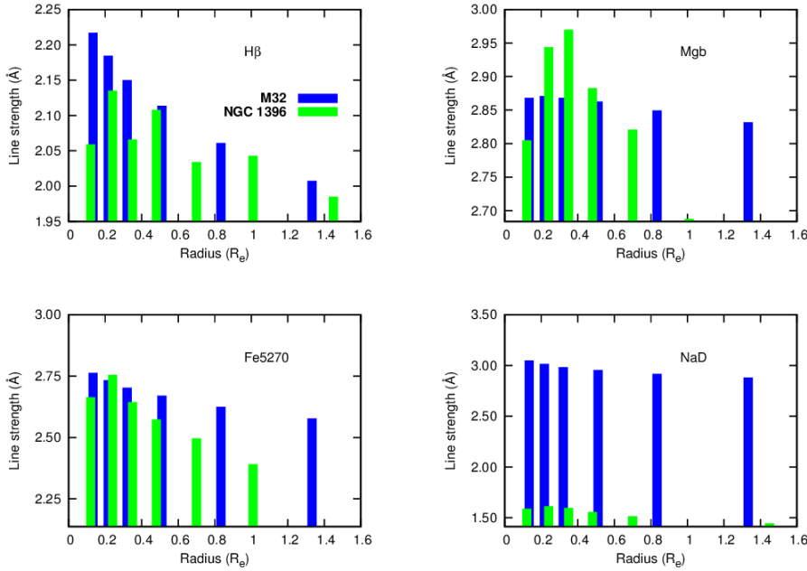
Figure 16. Radial comparison of the Lick indices H\beta , Mgb, Fe5270 and NaD, between NGC 1396 and M32. Line strengths from M32, measured at Lick resolution, are obtained from Worthey (2004), and converted to LIS 5.0 Å.
