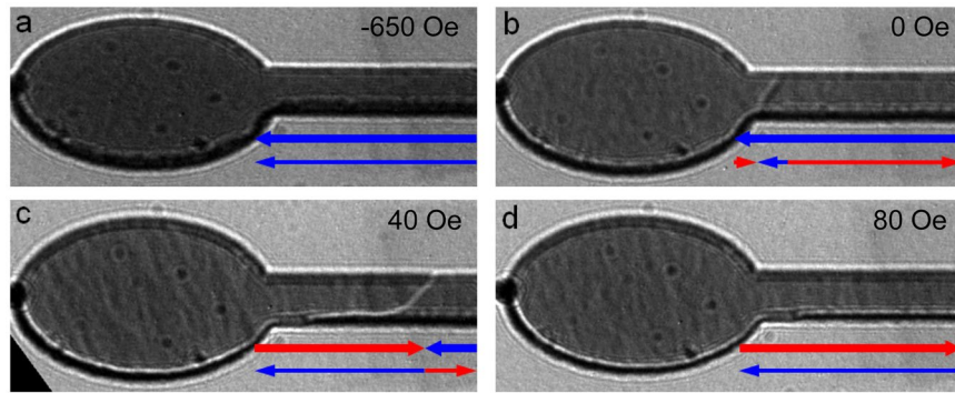
Figure 2. LTEM images of SyF nanowire with 800 nm wide track. The sequence of images shows the reversal of the ellipse and nucleation of a 180° AFM DW. The layers are t_1 = 13.3 nm and t_2 = 6.6 nm thick separated by a 0.7 nm thick Ru spacer layer. The transmission images contain contrast that arises as a projection of both layers. The images are taken for applied in-plane horizontal fields of (a), -650 Oe, saturation state, (b) 0 Oe, ellipse reversed and 360° wall formed in the thinner \text{Co}_{90}\text{Fe}_{10} layer, (c) 40 Oe, 180° AFM DW formed, and (d) 80 Oe, AFM DW removed. The red and blue arrows indicate the inferred direction of the magnetisation in each layer, with the thick/thin arrows representing the thicker (top) and thinner (bottom) layer respectively.
