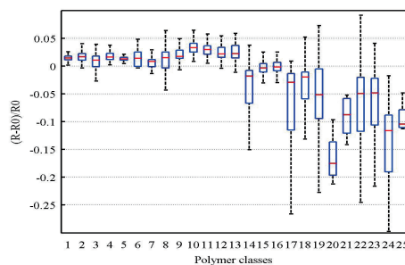
Fig.2. Boxplot of the steady state response of the sensors to a fixed concentration of acetic acid.
