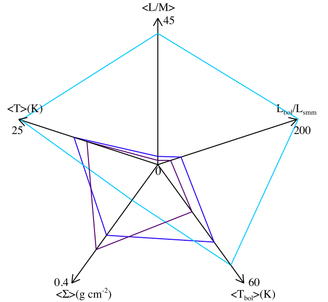
Figure 24. As in Fig. 23, but for protostellar sources (blue line) and for the two extracted populations of MIR-dark sources (dark-purple line) and H II-region candidates (light-blue line), respectively.
