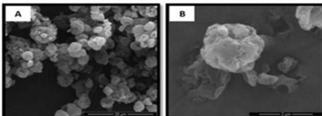
Fig. 1. SEM pictures of spraydried NPs/NCMPs. Scale bar (A) 20 \mu m and (B) 2 \mu m.
