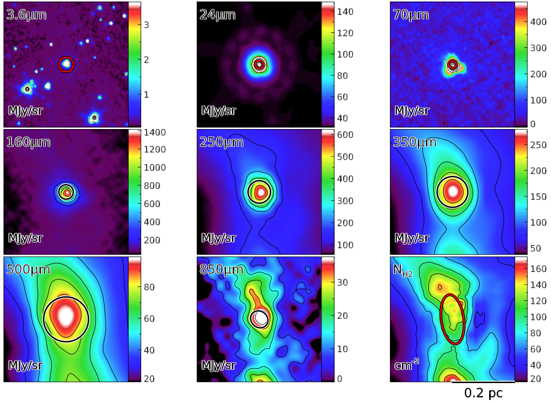
Fig. D.1. Images of a probable protostellar core in the Monoceros R2 region at 3.6 \mu\text{m} (IRAC), 24 \mu\text{m} (MIPS), 70 \mu\text{m} , 160 \mu\text{m} (PACS), 250 \mu\text{m} , 500 \mu\text{m} (SPIRE), 850 \mu\text{m} (SCUBA-2) and in the high-resolution column density map (source HOBYS J060711.2 –054721; number 144 in the full catalogue). All images cover the same spatial scale (approximately 100'' \times 100'' , or 0.4 \text{ pc} \times 0.4 \text{ pc} ); this is for consistency across all sources, some of which are much larger than HOBYS J060711.2 –054721. The ellipses show the extent of the source FWHM (assuming a 2d Gaussian shape) as determined by getsources for each individual wavelength. A black ellipse indicates that the detection at this wavelength was either considered reliable (160–850 \mu\text{m} ), or was a 70 \mu\text{m} detection used for the SED fit. (The ellipse shown at 3.6 \mu\text{m} is the ellipse measured at the reference wavelength; here 160 \mu\text{m} .) The source mass and angular size at the reference wavelength are given at the upper right of the snapshots. We note that only one set of snapshots is included here; the full catalogue will contain snapshots for all robust sources. The SED of this source is given in Fig. D.2.
