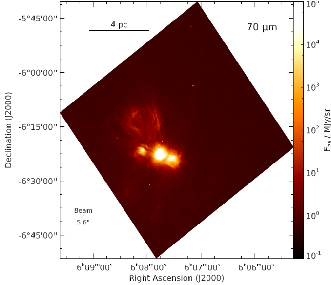
Fig. A.1. Monoceros R2 as viewed by Herschel PACS 70\ \mu\text{m} . The image is 1.15^{\circ} \times 1.3^{\circ} ( 16.7 \times 19.1 pc) in size. The diffraction-limited instrumental beam ( 5.6'' ) is shown to the lower left of the image.
