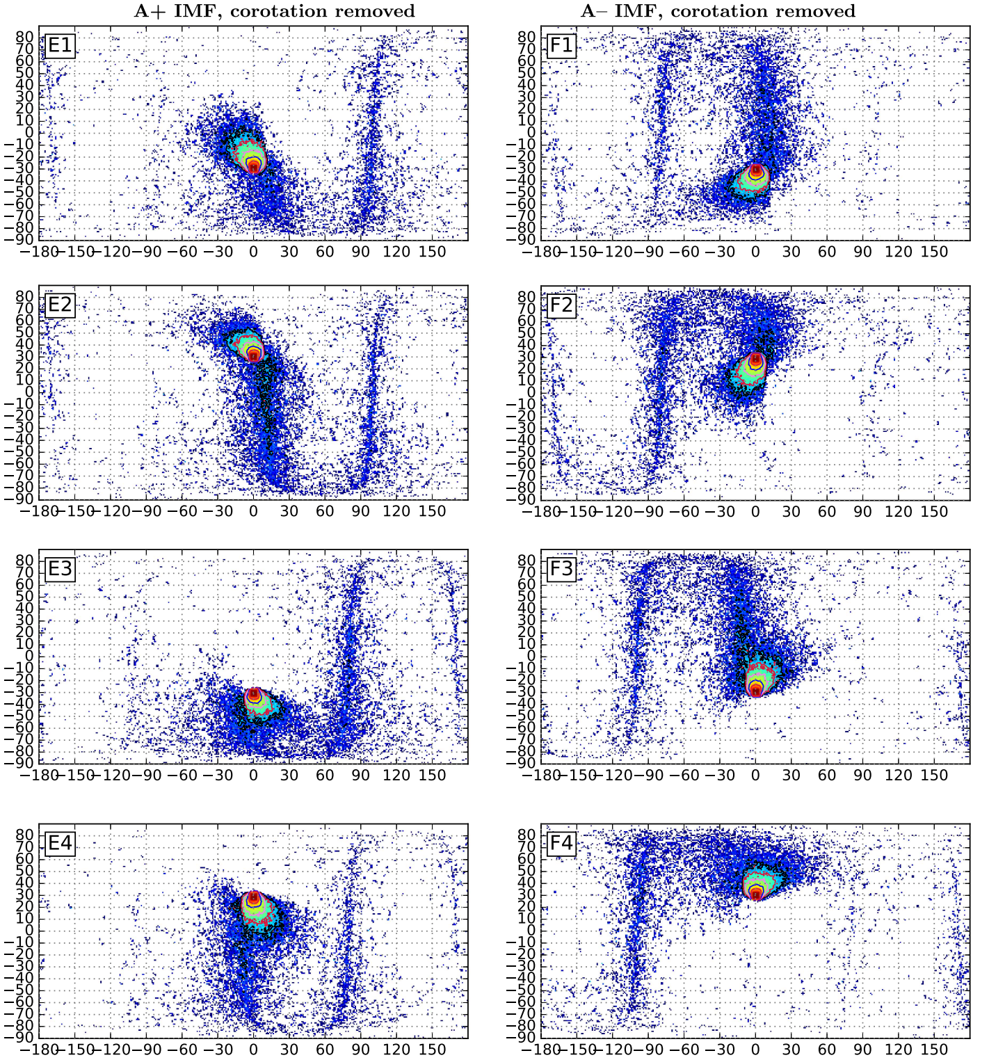
Figure 3. Fluence maps of protons, injected from a power law with \gamma = -1.1 , spanning the energy range from 10 to 800 MeV, crossing the 1 au sphere, over a time of 100 hr. Effects of corotation are removed. Fluence colors are on a logarithmic scale, overlaid by contours, two per decade. Injection regions were 6^\circ \times 6^\circ . Panels are labeled E1 through F4 according to simulation setup, with dipole tilt angles of 85^\circ , representing a case of significant solar activity.
