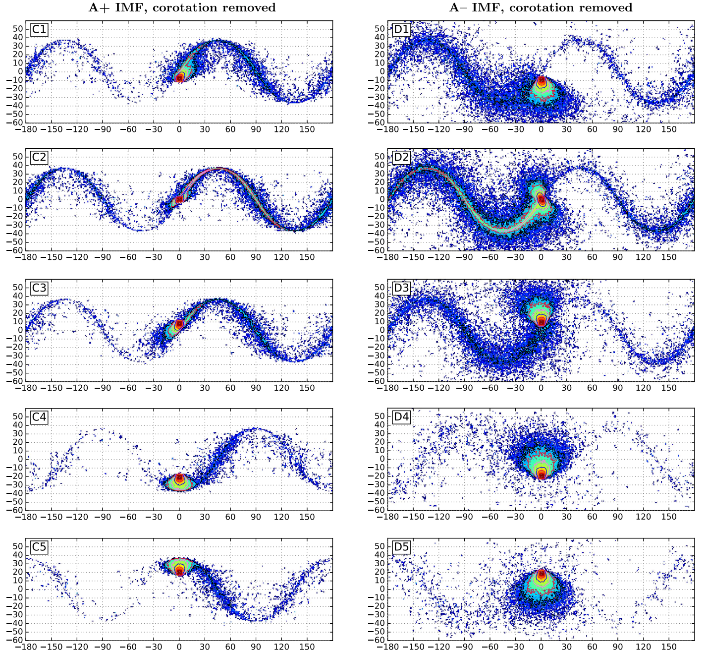
Figure 2. Fluence maps of protons, injected from a power law with \gamma = -1.1 , spanning the energy range from 10 to 800 MeV, crossing the 1 au sphere, over a time of 100 hr. Effects of corotation are removed. Fluence colors are on a logarithmic scale, overlaid by contours, two per decade. Injection regions were 6^\circ \times 6^\circ . Panels are labeled C1 through D5, according to simulation setup.
