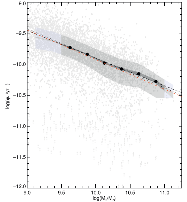
Figure 2. sSFR \psi_* as a function of stellar mass M_* for the FCS sample. Values for individual sample galaxies are shown as grey circles, with downward arrows indicating those galaxies for which the derived value of \psi_* is an upper limit (at 2.5\sigma ; as discussed in detail in Paper I, the depth of the GALEX–GAMA UV data is such, that the second quartile and the median are defined by detections). The median \psi_* – M_* relation in bins of 0.25 dex in M_* is shown by the transparent shaded regions, with the width of the darker narrower region indicating the bootstrapped uncertainty in the median, and the width of the wider, lighter region indicating the interquartile range. Given the mass limit of M_* \geq 10^{9.5} to which the FCS sample is volume complete, and the low number of sources with M_* \geq 10^{11} M_\odot , we have fit a single power law \log(\psi_*) = A + \gamma(\log(M_*) - 10) to the binwise median values denoted by the black filled circles, denoted by the black dash–dotted line. For comparison, the empirical parametrization of the main sequence of star-forming galaxies presented by Speagle et al. (2014), extrapolated to the median redshift of the FCS sample of z = 0.1 , is shown as a red dashed line, while a black dotted line shows the result of fitting power law with the slope fixed to the expectation value for the main sequence.
