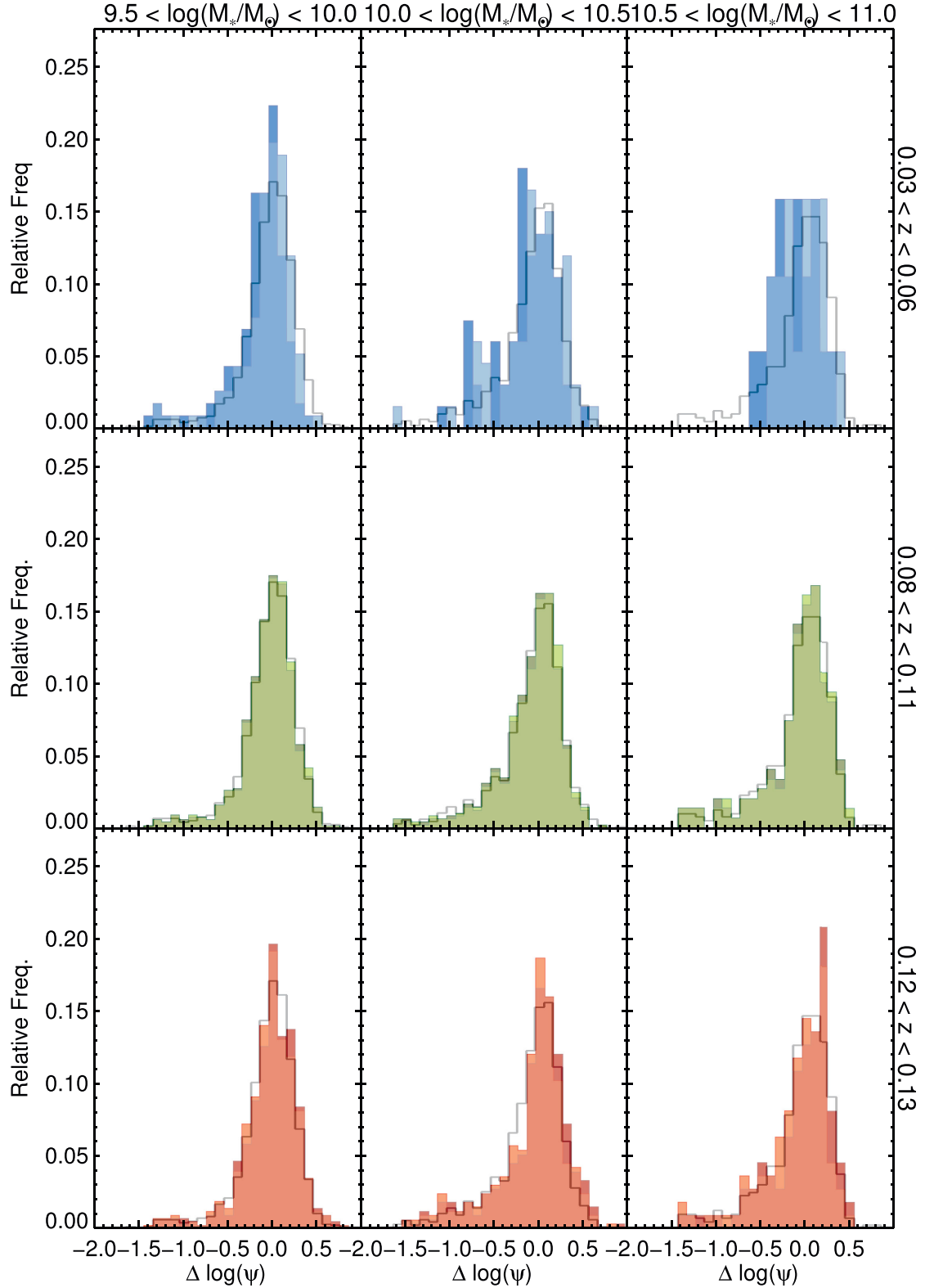
Figure 4. Evolution of \Delta \log(\psi_*) for the z_1 , z_2 , and z_3 sub-samples of the FCS sub-sample (top to bottom) in three bins of stellar mass M_* as indicated (left to right). The mass range encompasses \gtrsim 99 per cent of the FCS sample. The distribution of \Delta \log(\psi_*) in each mass bin for the full FCS sample is shown as a grey solid line, while the distributions of \Delta \log(\psi_*) for the redshift subsamples are shown as dark shaded histograms and the distributions of \Delta_{z_i} \log(\psi_*) are shown as lighter shaded histograms. Quantitative statistical tests of the similarity of the distributions within each stellar mass bin are listed in Table 3.
