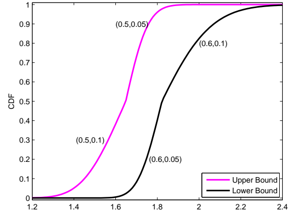
Fig. 2. P-box for event X
