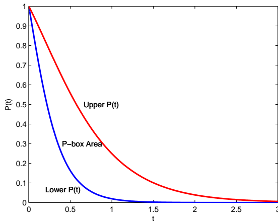
Fig. 3. Example of p-box of the system survival function
