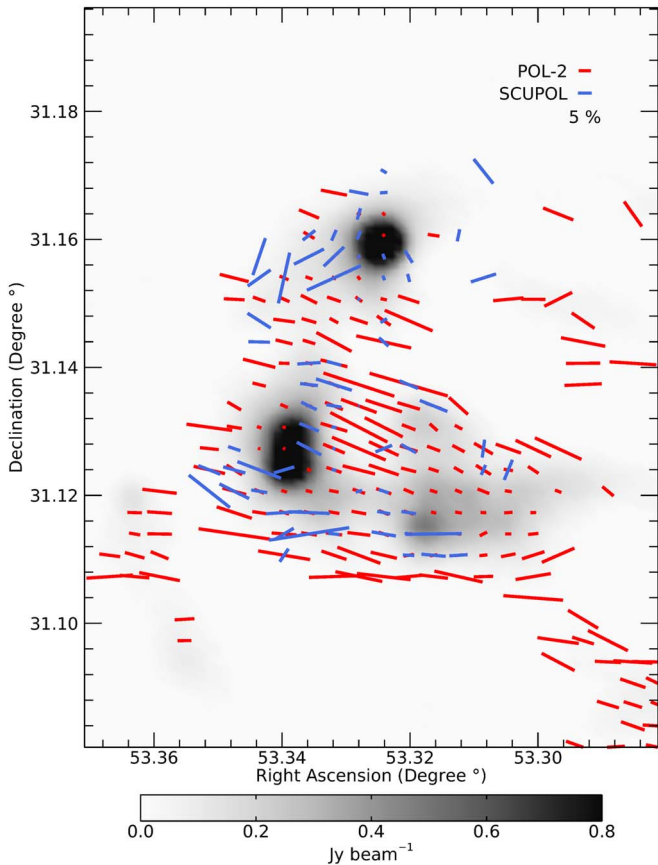
Figure 4. Comparison of dust polarization at 850\ \mu\text{m} between POL-2 (red) and SCUPOL (blue) toward Perseus B1. The gray scale indicates the Stokes I total intensity measured with POL-2. The length of each vector is determined by its associated polarization fraction P (percent). The SCUPOL polarization vectors from Matthews et al. (2009) have been rebinned to match the exact position and pixel scale (from 10'' to 12'' ) of the POL-2 observations.
