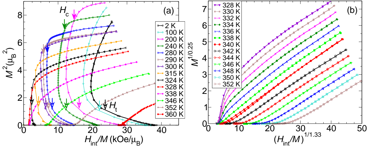
FIG. 3. (Color online) (a) Standard Arrott plot with corrected M(H) curves (per f.u.) measured at selected temperatures. Points corresponding to magnetic fields H_t and H_c at different temperatures are indicated by open and filled arrows, respectively. (b) Modified Arrott plot with critical exponents \beta = 0.25 and \gamma = 1.33 applied to get straight lines in the high field range.
