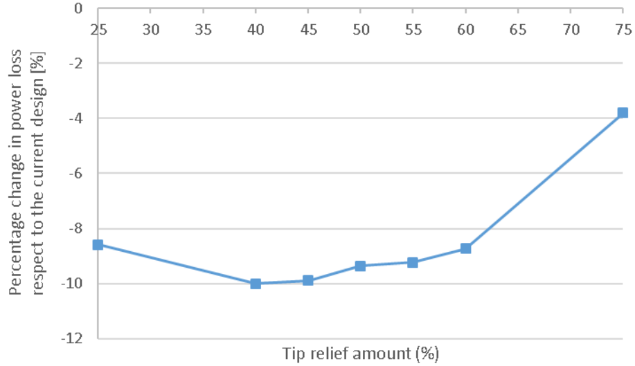
Figure 9: Percentage change in power loss with respect to the current design for 25% - 75% tip relief amount (with surface roughness of 1.6 μm)
