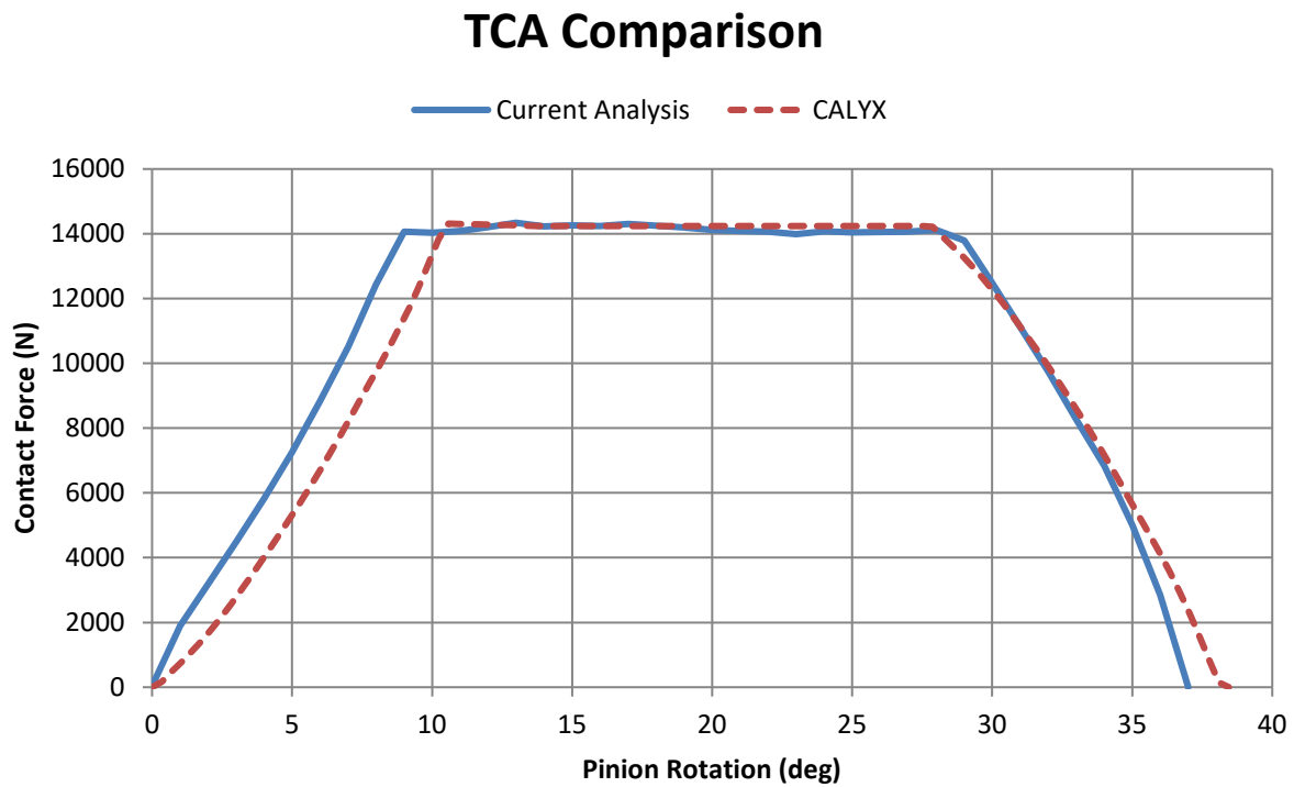
Figure 5 – Current Analysis and CALYX TCA Force Comparison
