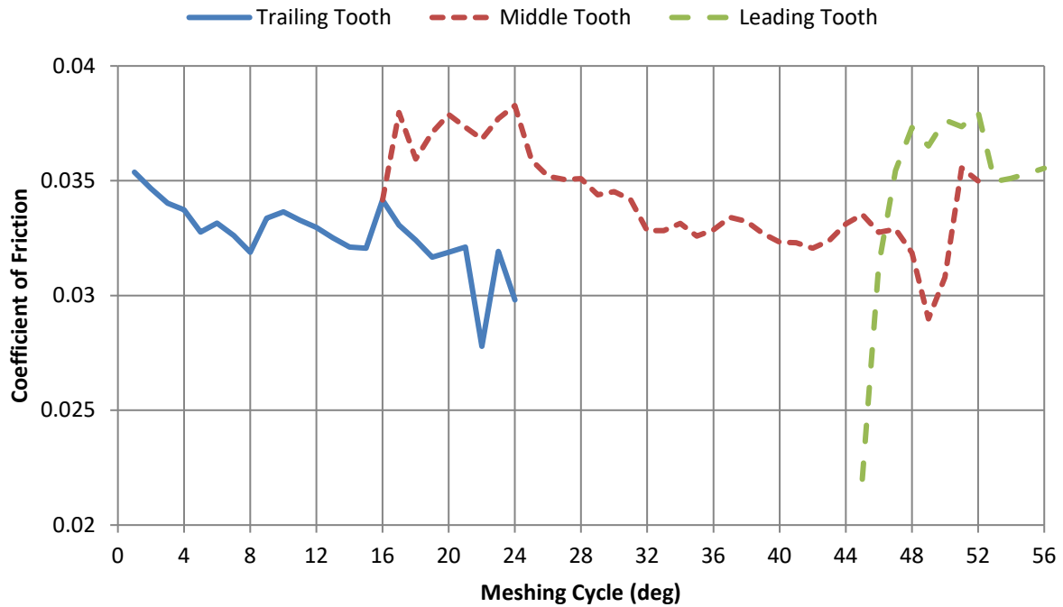
Figure 9 - Coefficient of Friction through meshing cycle
