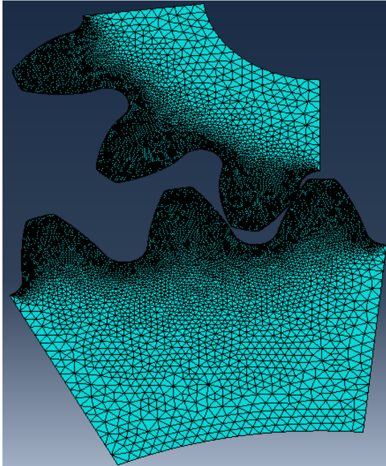
Figure 2 - Gear Assembly Meshed (Front Face)
