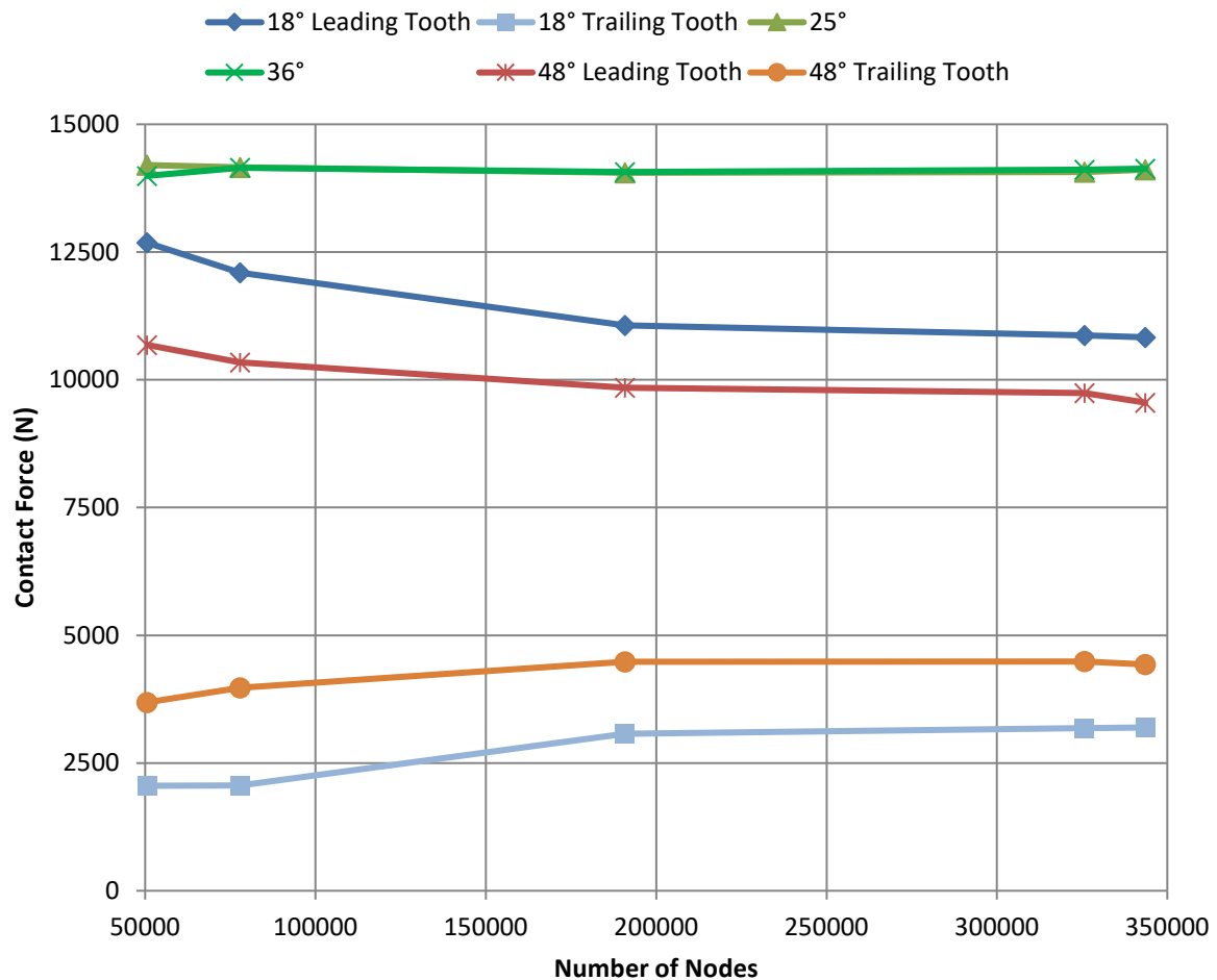
Figure 6 - Mesh Sensitivity at 18, 25, 36 and 48°
