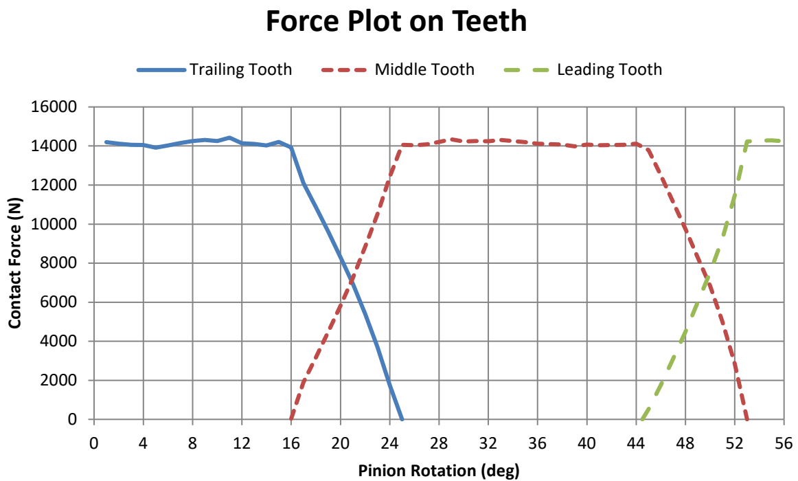
Figure 4 - Tooth contact force variation through meshing cycle
