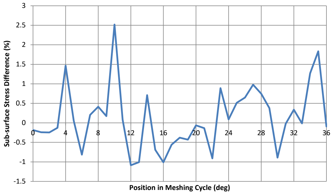
Figure 10 - Maximum sub-surface stress difference between 'LTCA' and 'LLTCA' analyses
