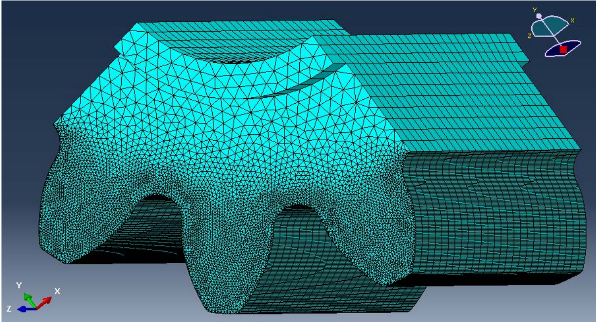
Figure 3 - Pinion Mesh (Isometric)
