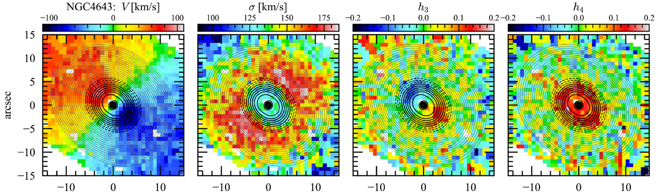
Figure 16. A close-up of the lower panels (ATLAS 3D stellar kinematics) of Fig. 15, but with contours now showing the ratio of the nuclear-disc component to the rest of our best-fitting model of NGC 4643 (e.g. Fig. 10). Solid black contours indicate where the nuclear disc is brighter, dashed black contours where its brightness is 50–100 per cent of the rest of the model, and thin grey contours where it is fainter. Note that the region dominated by the nuclear-disc component matches almost perfectly with the fast rotation, lower velocity dispersion, strong V – h_3 anticorrelation, and enhanced h_4 .
