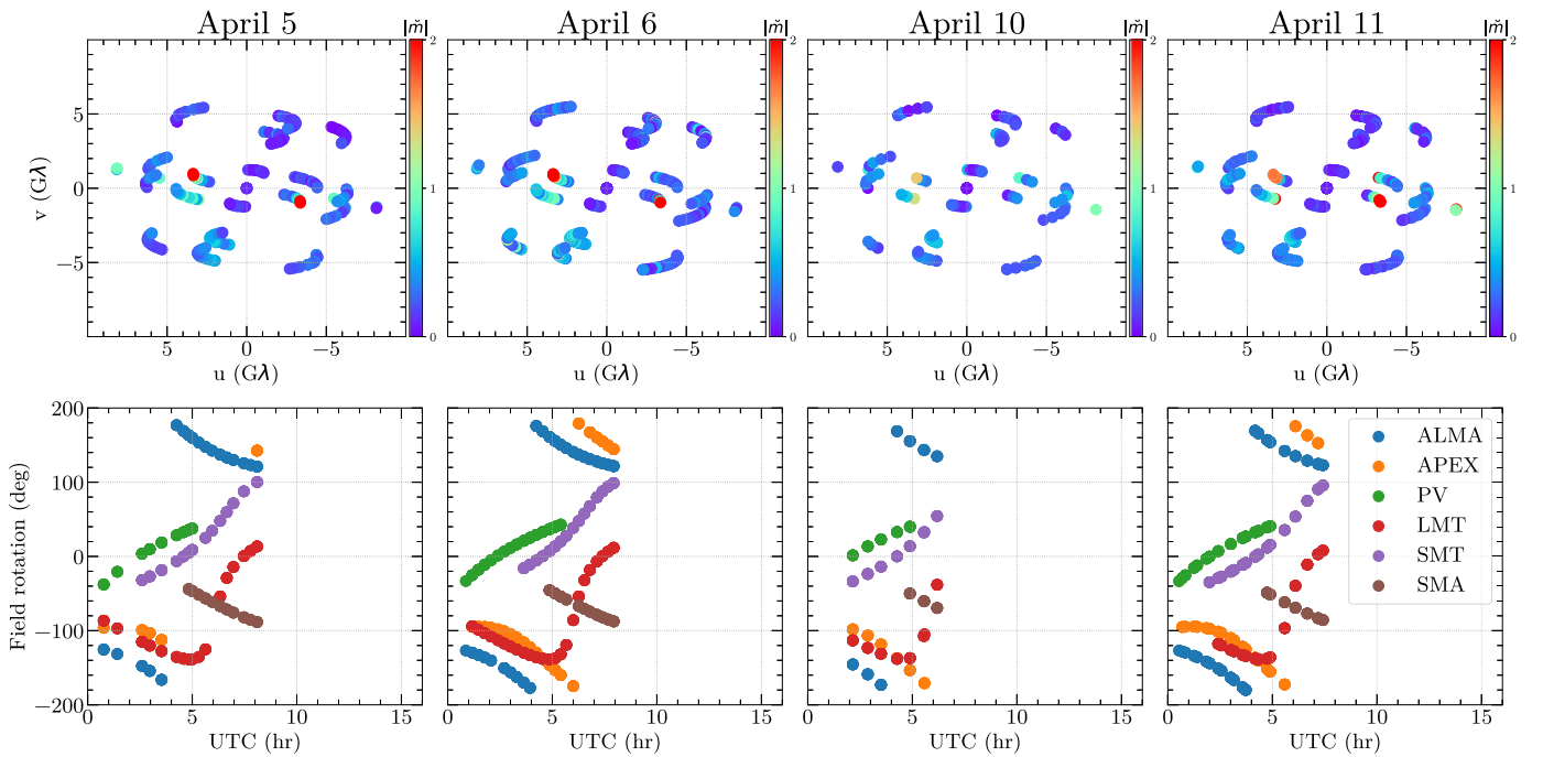
Figure 1. Top row: (u, v) coverage of the four M87 observing days in the 2017 campaign. The color of the data points codes the fractional polarization amplitude |\check{m}(u, v)| in the range from 0 to 2. The data shown are derived from low-band visibilities after the initial calibration pipeline described in Section 3.2 but before any D-term calibration. The data points are coherently scan-averaged. Bottom row: M87 field rotation angle \phi for each station as a function of time (Equation (5)).
