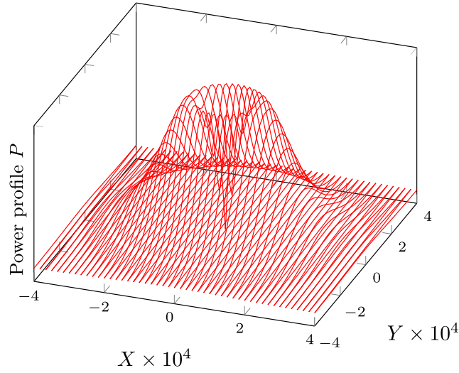
Figure 1. Power profile P of the (CM,1) laser pulse at Z = 0, T = 0 with parameters \{\Lambda = 600, \Psi_1 = 1, \Psi_2 = 1000, \Phi = 0.001, \Xi = 1\} . Reproduced with permission by [30]. Copyright 2016 Elsevier.
