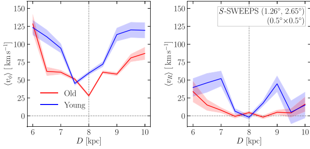
Figure 6. LOS profiles of galactocentric ( \langle v_\phi \rangle ) (left-hand panel) and ( \langle v_R \rangle ) (right-hand panel) for the S -SWEEPS field in the model.
