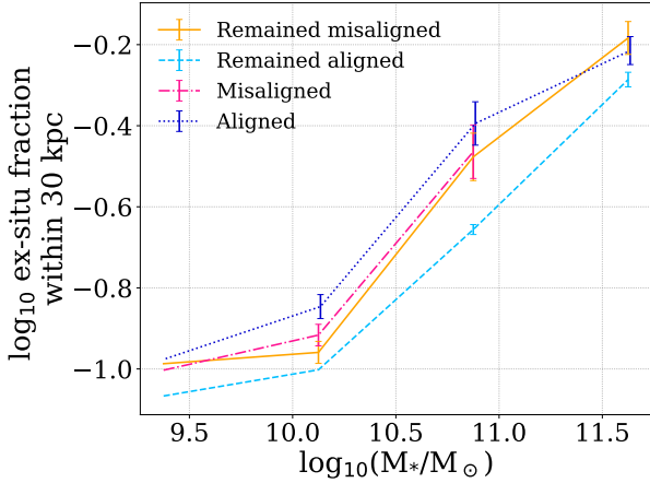
FIGURE 12. Distribution of ex-situ stellar fraction in stellar mass bins for each population described in Table 1 at z = 0.0 - 0.1 . Only bins with more than five galaxies are shown. Error bars are Poisson errors.
