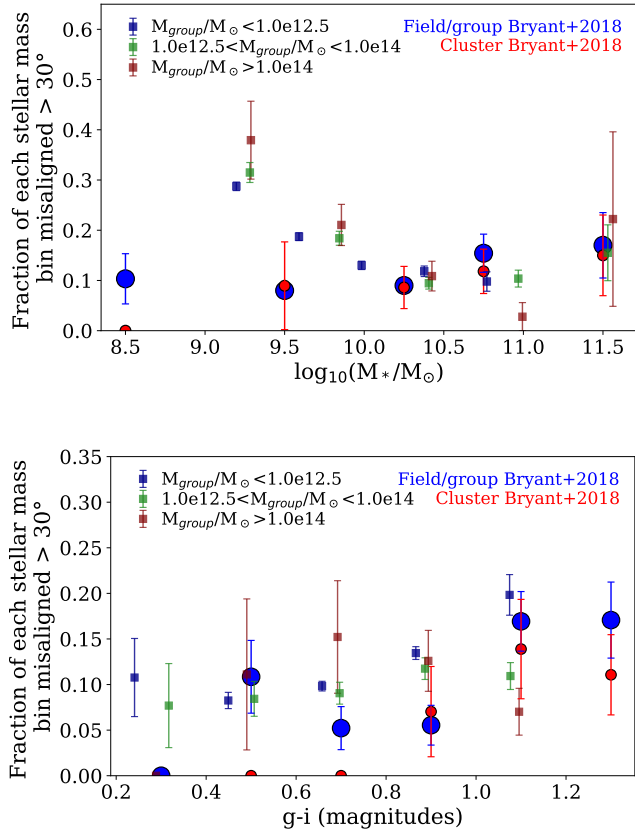
FIGURE 3. Fraction of galaxies that are misaligned (PA offset > 30^\circ ) in bins of stellar mass (top panel) and in bins of g-i colour (bottom panel). The circles are the results obtained with EAGLE simulated galaxies and the squares are the results of Bryant et al. (2018), using SAMI. Our sample is separated into three ranges in halo mass, as labeled. Simulated data errors correspond to Poisson uncertainties.
