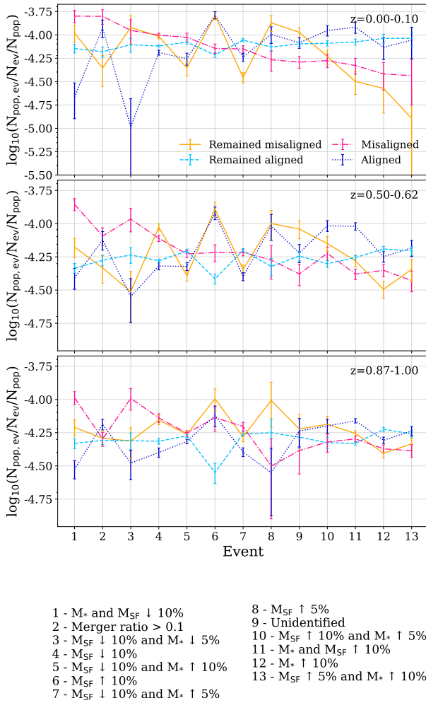
FIGURE 15. Number of galaxies of each population associated with an event ( N_{pop,ev} ), over the total number of galaxies that experienced that event ( N_{ev} ), and over the total number of galaxies in that population ( N_{pop} ), at three redshift ranges (as labelled on each panel). The integers on the x-axis correspond to each event listed below the figure. Error bars are Poisson errors.
