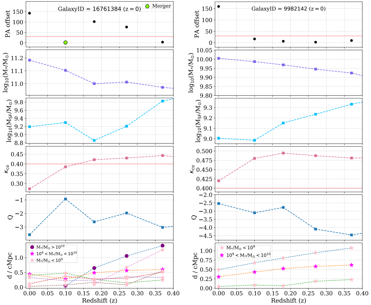
FIGURE 13. From top to bottom, we show the evolution through redshift for two galaxies of PA offset between the rotational axes of the stars and star-forming gas (the red dashed line marks 30^\circ ), stellar mass, star-forming gas mass, stellar co-rotating kinetic energy fraction (the red dashed line marks \kappa_{\text{co}} = 0.4 ), tidal strength parameter Q , and the distance with neighboring galaxies when the misalignment occurs (closer than 0.7 \text{ cMpc} ), colored by mass ranges. In the upper panel on the left, the green dot indicates where the merger occurred.
