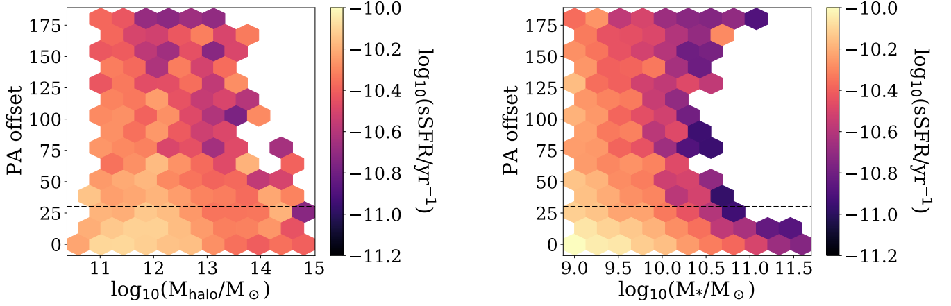
FIGURE 7. Binned distribution of the angle between the stellar and star-forming gas angular momentum vectors versus halo mass of the group in which the galaxy resides (left panel) and versus the stellar mass (right panel) coloured by the average Log sSFR, as shown in the colour bar, for galaxies at z = 0.0 - 0.1 . Only bins with more than five galaxies are shown. The black dashed lines mark a PA offset = 30^\circ to separate between aligned and misaligned galaxies.
