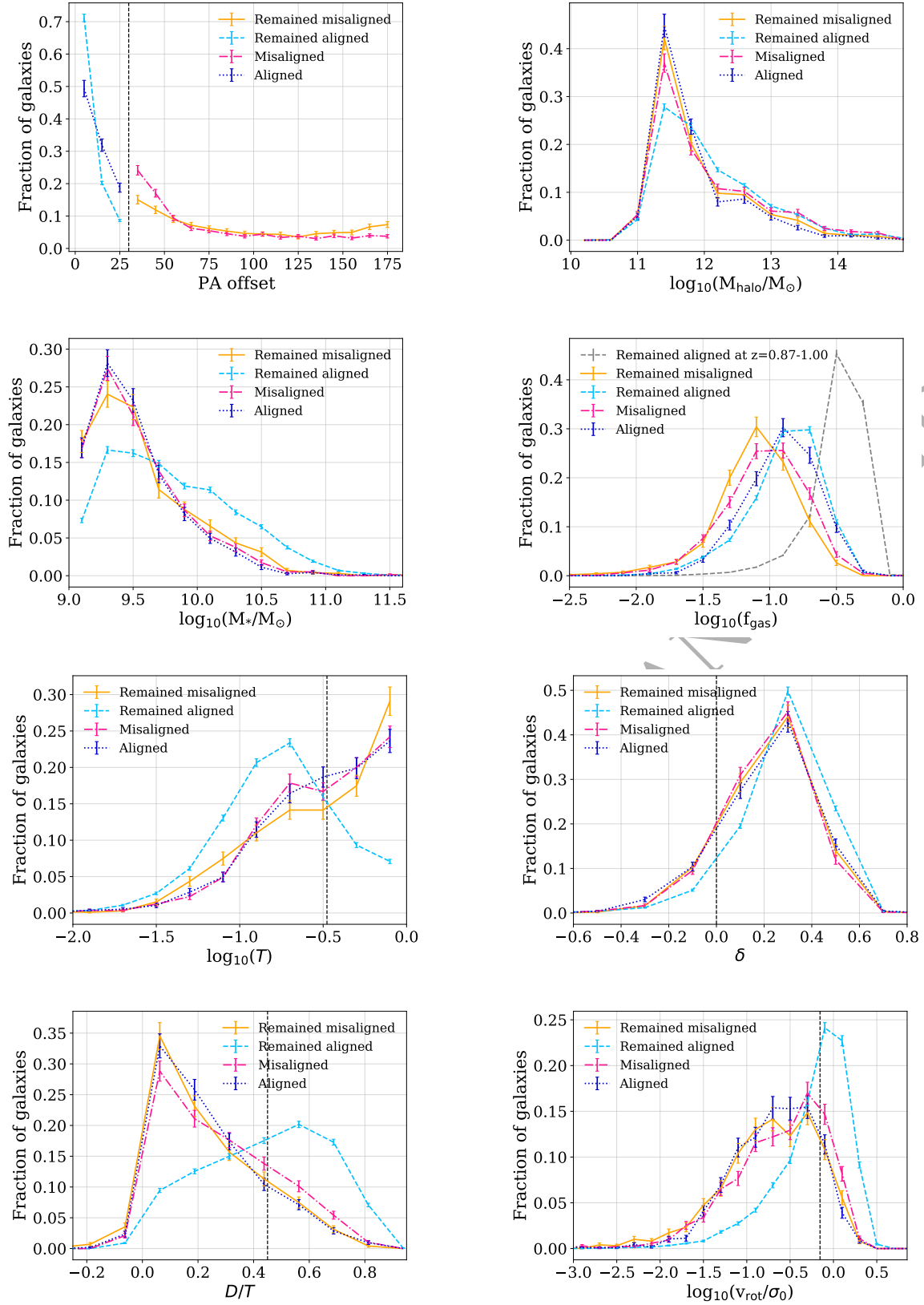
FIGURE 9. Each panel shows the distribution of galaxy properties normalized to each population described in Table 1 at z = 0.00 - 0.10 . From top left and counterclockwise, galaxy properties are : gas-stellar position angle offset, stellar mass, triaxiality parameter (the black dashed line marks T=1/3 to separate between oblate and prolate systems), the disc-to-total stellar mass ratio (the black dashed line signalize D/T = 0.45 to divide between star-forming and passive galaxies), the ratio between the stellar rotational velocity and the velocity dispersion (the black dashed line marks v_{\text{rot}}/\sigma_0 = 0.7 to separate between star-forming and passive galaxies), stellar velocity anisotropy parameter, gas fraction, and halo mass. The fractions in each bin sum to 1. Errors correspond to Poisson uncertainties.
