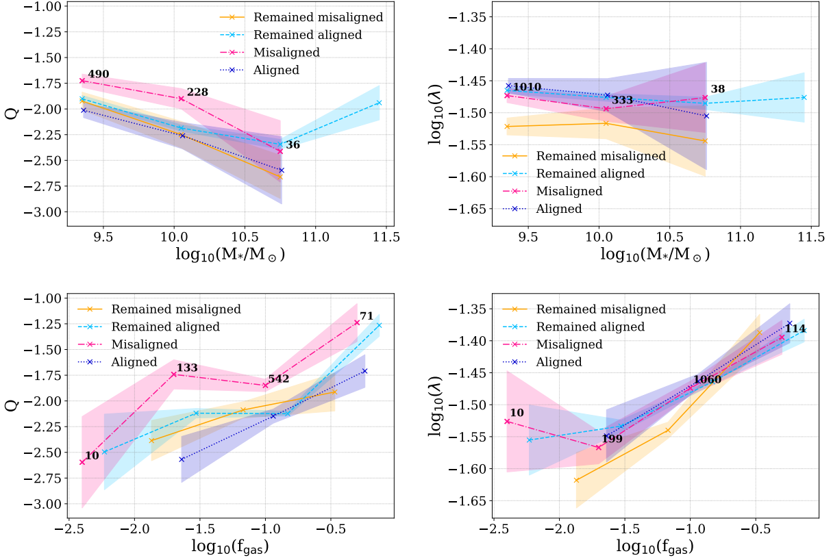
FIGURE 11. Left panels show the average tidal strength parameter Q in bins of stellar mass (top panel) and bins of gas fraction (bottom panel) for each population described in Table 1 at z = 0.00 - 0.10 . Same for right panels but for the halo spin parameter \lambda . The number of galaxies considered in each bin for the ‘misaligned’ population is shown, and the shaded area represents the Poisson error.
