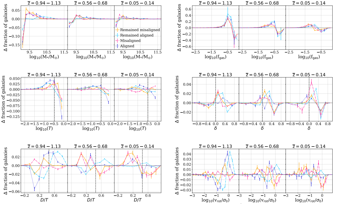
FIGURE 10. Each chart shows the difference in the abundance of galaxies in each bin between two consecutive snapshots. We show this for all the properties studied in Fig. 9. A positive/negative value of ‘ \Delta fraction of galaxies’ means that the number of galaxies increases/decreases in each galaxy property bin, between two consecutive snapshots. Errors correspond to Poisson uncertainties.
