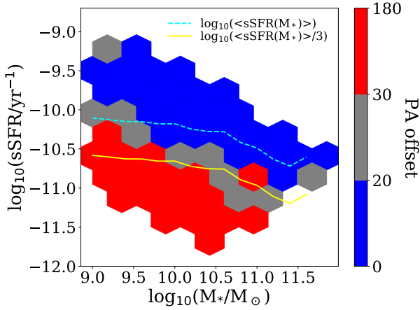
FIGURE 8. Binned distribution of galaxies in the sSFR- M_* plane coloured by the average gas-stellar position angle offset at z = 0.0 - 0.11 . The dashed blue line marks the main sequence of star formation and solid yellow line separates the population between blue cloud and red sequence. Only bins with more than five galaxies are shown.
