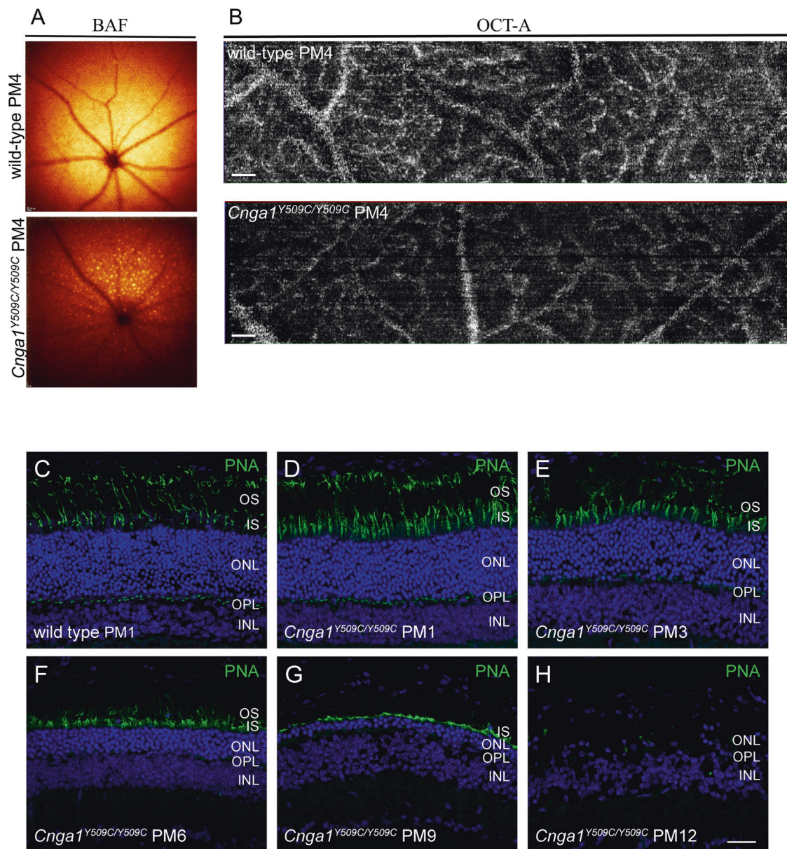
Fig. 7 Cnga1 Y509C/Y509C mice show secondary retinal morphological changes and degeneration of cone photoreceptors. Representative BAF and OCT-A scans of the fundus (A) and retinal vasculature (B) showing accumulation of autofluorescent spots and altered vascular bed in the Cnga1 Y509C/Y509C mouse fundus. Representative confocal images showing expression of peanut agglutinin (PNA; green) in retinal cross sections of wild-type (1 month postnatal (PM1); (C) and Cnga1 Y509C/Y509C mouse retinas (D–H) at PM1, PM3, PM6, PM9 and PM12 demonstrating a degeneration of cone photoreceptors with age. Scale bars in B marks 200 μm. Scale bar in H marks 25 μm.
